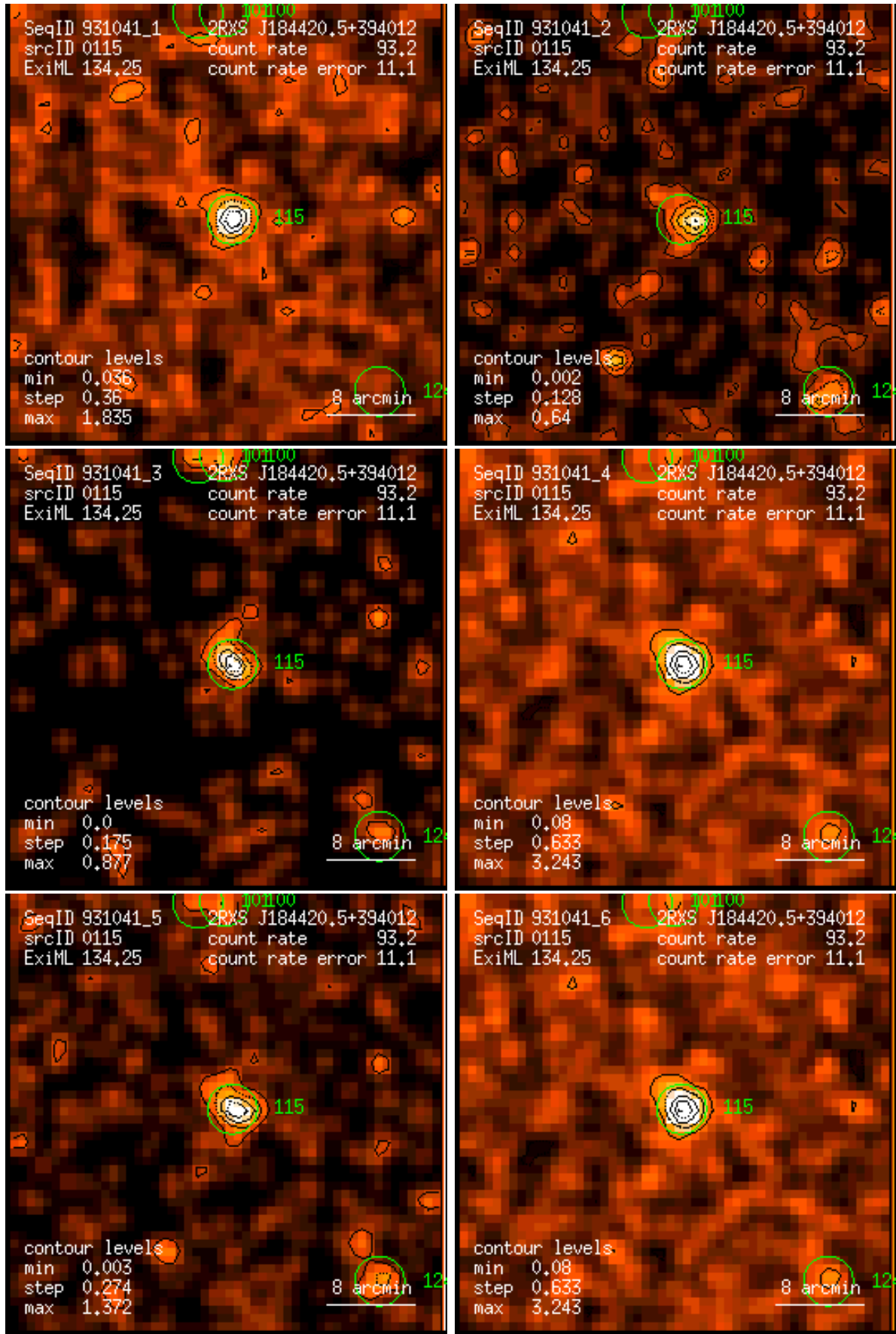
Figure 115: RASS 931041: detection 0115: band rate images, Gaussian filter: (1) PSPC channels 11 – 41, (2) 52 – 90, (3) 91 – 201, (4) 11 – 235, (5) 52 – 201, (6) 11 – 201. Broad band rates in counts/ks. Band rate contour levels in counts/ks/arcmin 2 .
