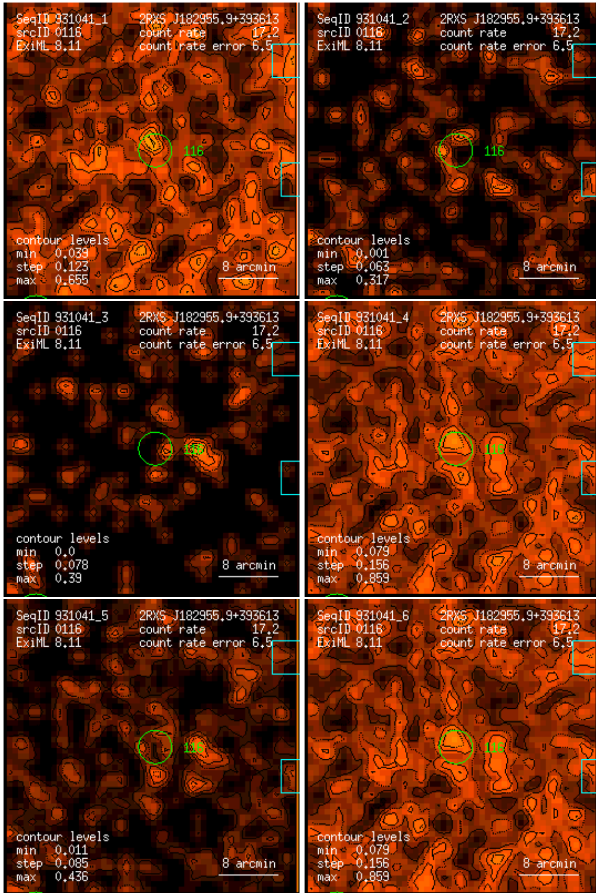
Figure 116: RASS 931041: detection 0116: band rate images, Gaussian filter: (1) PSPC channels 11 – 41, (2) 52 – 90, (3) 91 – 201, (4) 11 – 235, (5) 52 – 201, (6) 11 – 201. Broad band rates in counts/ks. Band rate contour levels in counts/ks/arcmin 2 .
