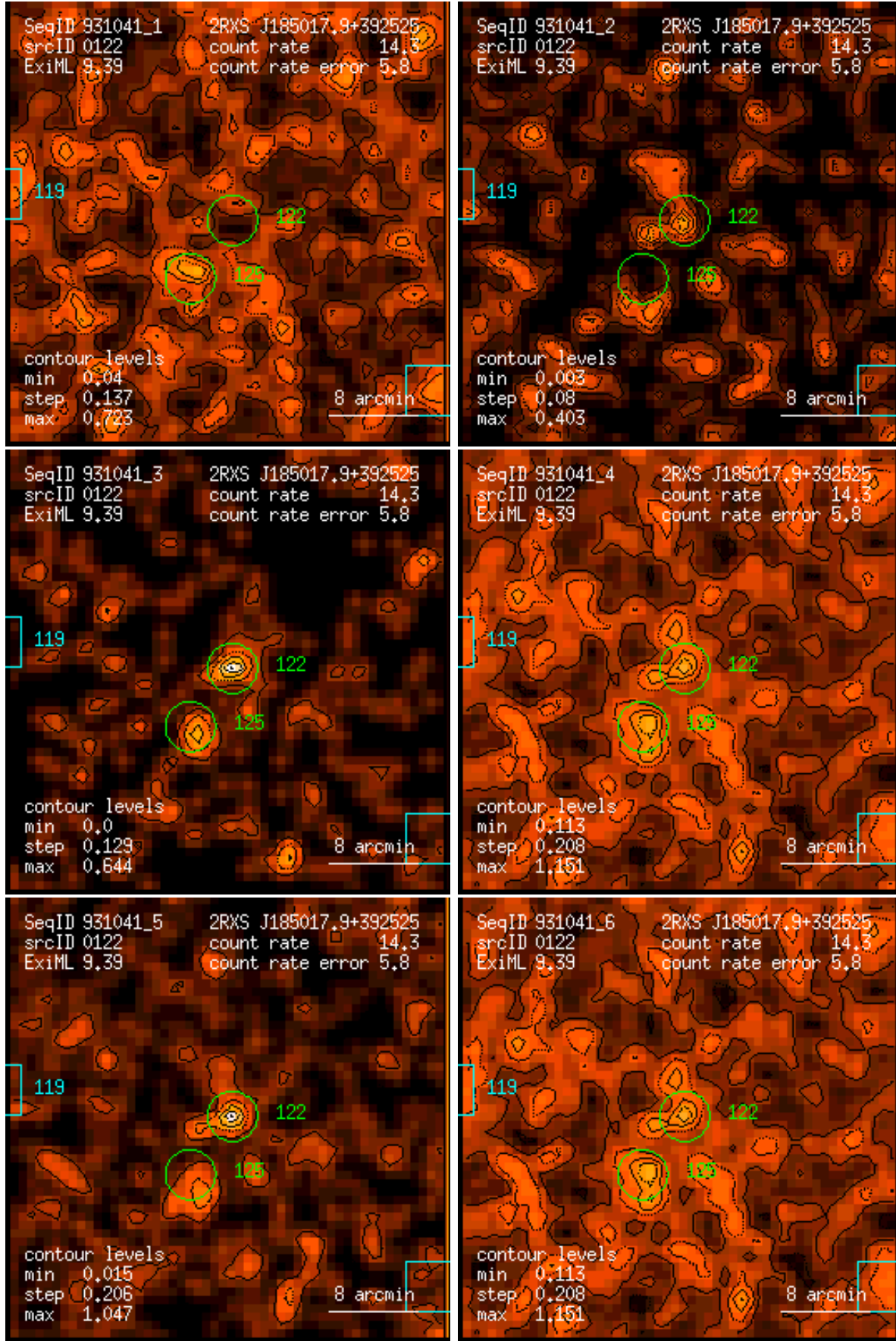
Figure 122: RASS 931041: detection 0122: band rate images, Gaussian filter: (1) PSPC channels 11 – 41, (2) 52 – 90, (3) 91 – 201, (4) 11 – 235, (5) 52 – 201, (6) 11 – 201. Broad band rates in counts/ks. Band rate contour levels in counts/ks/arcmin 2 .
