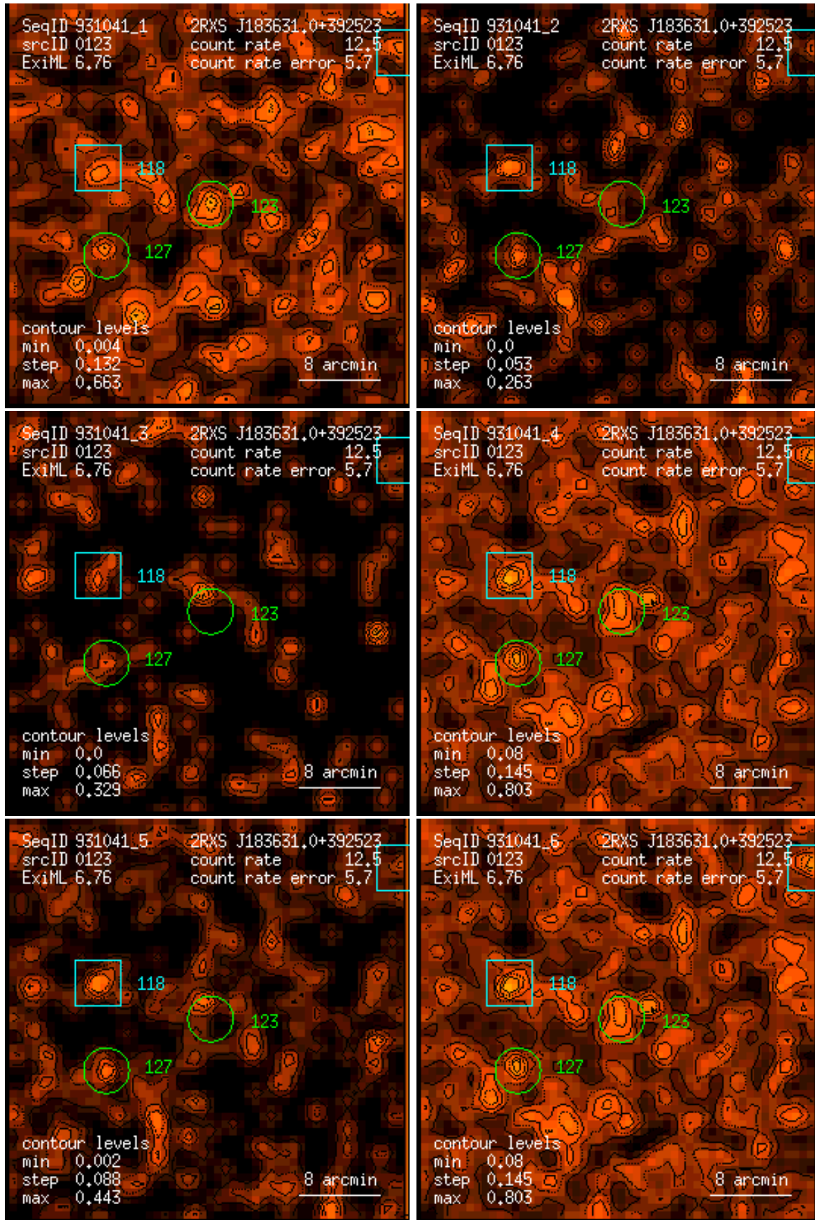
Figure 123: RASS 931041: detection 0123: band rate images, Gaussian filter: (1) PSPC channels 11 – 41, (2) 52 – 90, (3) 91 – 201, (4) 11 – 235, (5) 52 – 201, (6) 11 – 201. Broad band rates in counts/ks. Band rate contour levels in counts/ks/arcmin 2 .
