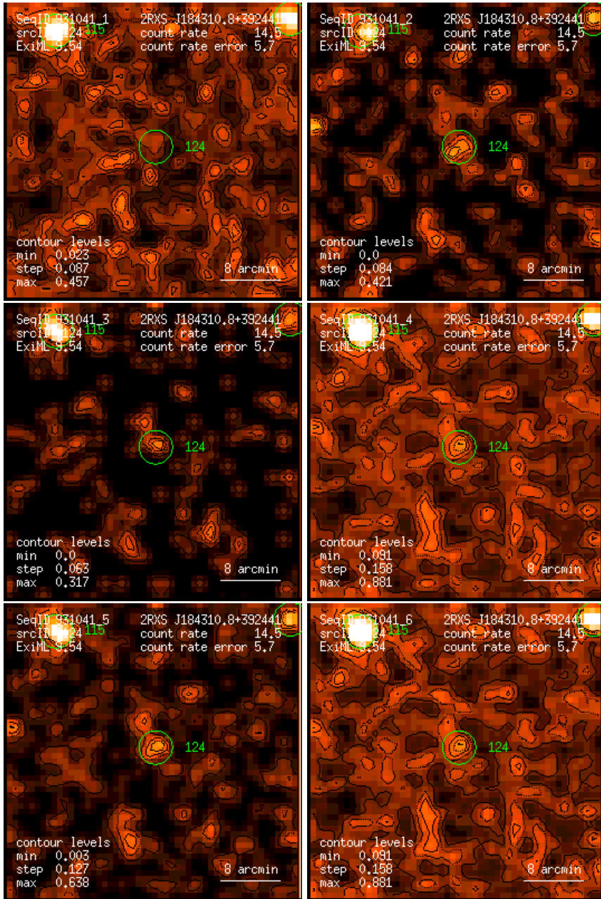
Figure 124: RASS 931041: detection 0124: band rate images, Gaussian filter: (1) PSPC channels 11 – 41, (2) 52 – 90, (3) 91 – 201, (4) 11 – 235, (5) 52 – 201, (6) 11 – 201. Broad band rates in counts/ks. Band rate contour levels in counts/ks/arcmin 2 .
