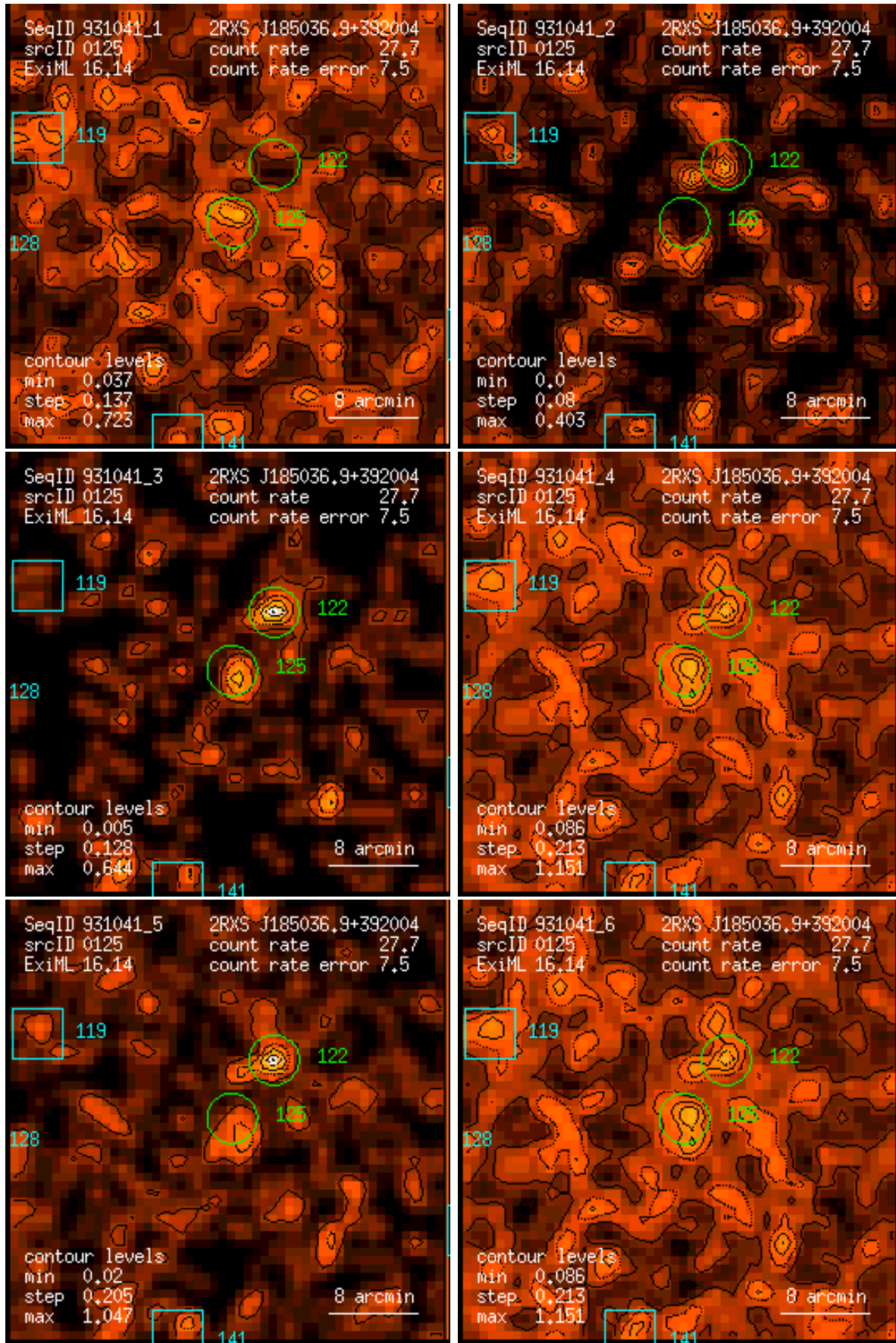
Figure 125: RASS 931041: detection 0125: band rate images, Gaussian filter: (1) PSPC channels 11 – 41, (2) 52 – 90, (3) 91 – 201, (4) 11 – 235, (5) 52 – 201, (6) 11 – 201. Broad band rates in counts/ks. Band rate contour levels in counts/ks/arcmin 2 .
