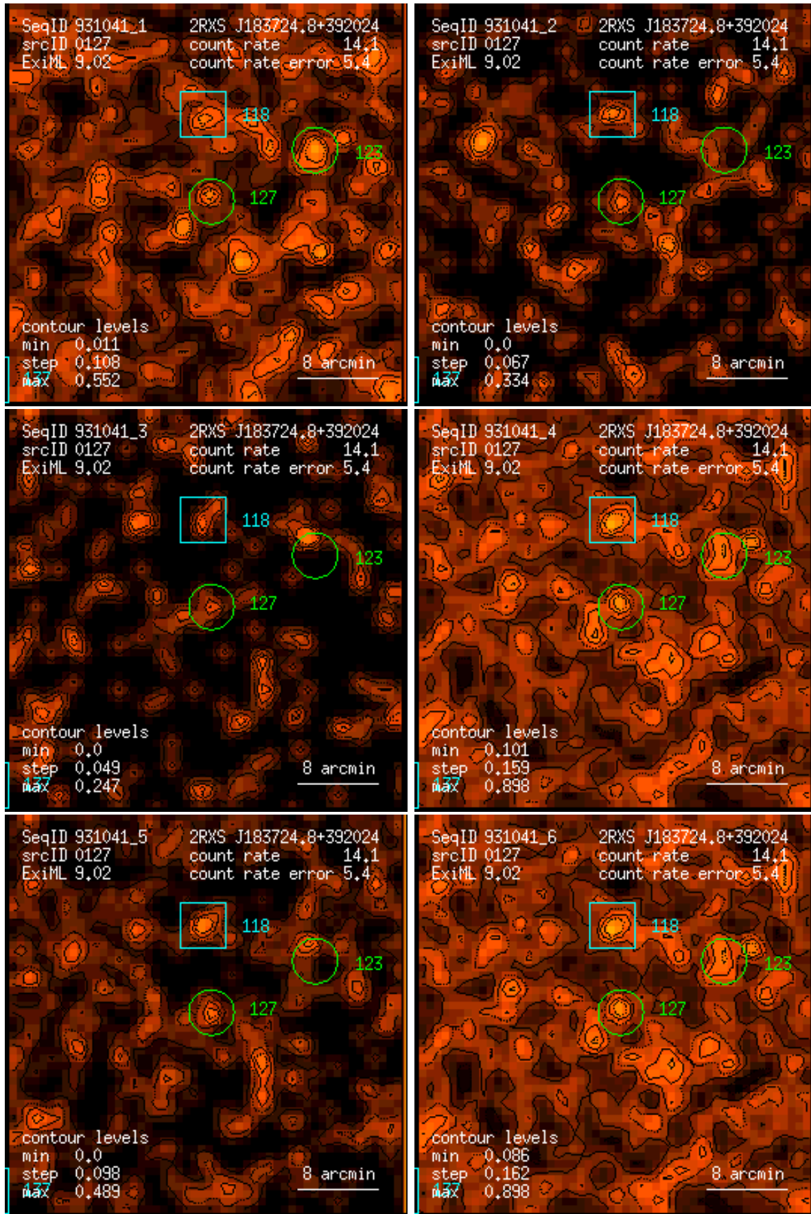
Figure 127: RASS 931041: detection 0127: band rate images, Gaussian filter: (1) PSPC channels 11 – 41, (2) 52 – 90, (3) 91 – 201, (4) 11 – 235, (5) 52 – 201, (6) 11 – 201. Broad band rates in counts/ks. Band rate contour levels in counts/ks/arcmin 2 .
