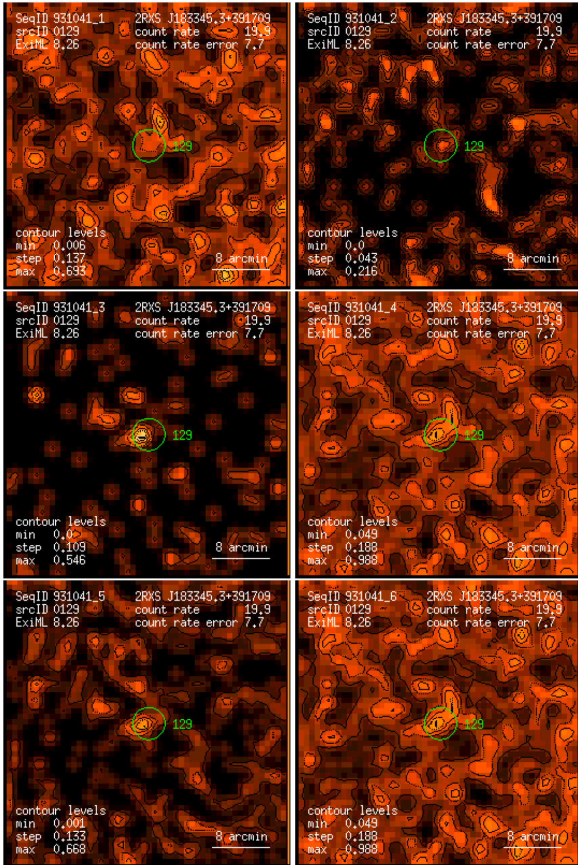
Figure 129: RASS 931041: detection 0129: band rate images, Gaussian filter: (1) PSPC channels 11 – 41, (2) 52 – 90, (3) 91 – 201, (4) 11 – 235, (5) 52 – 201, (6) 11 – 201. Broad band rates in counts/ks. Band rate contour levels in counts/ks/arcmin 2 .
