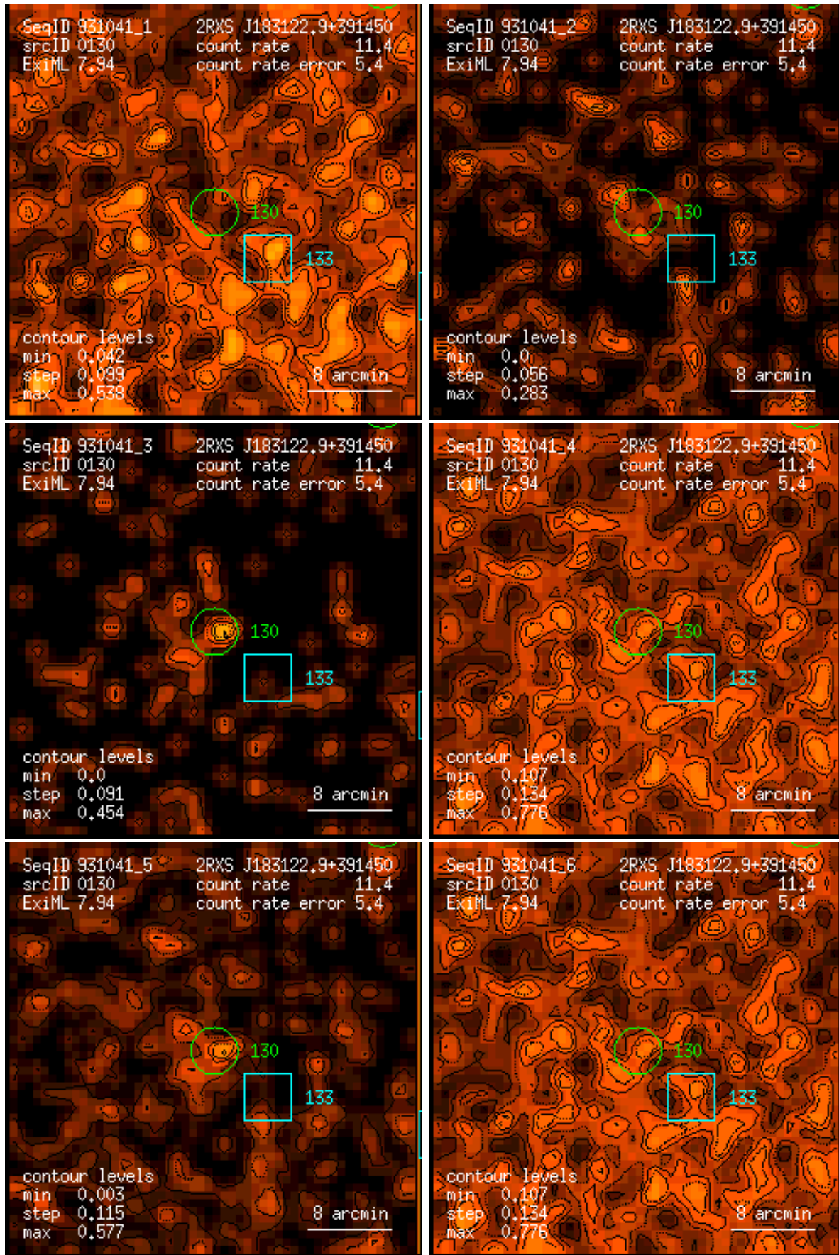
Figure 130: RASS 931041: detection 0130: band rate images, Gaussian filter: (1) PSPC channels 11 – 41, (2) 52 – 90, (3) 91 – 201, (4) 11 – 235, (5) 52 – 201, (6) 11 – 201. Broad band rates in counts/ks. Band rate contour levels in counts/ks/arcmin 2 .
