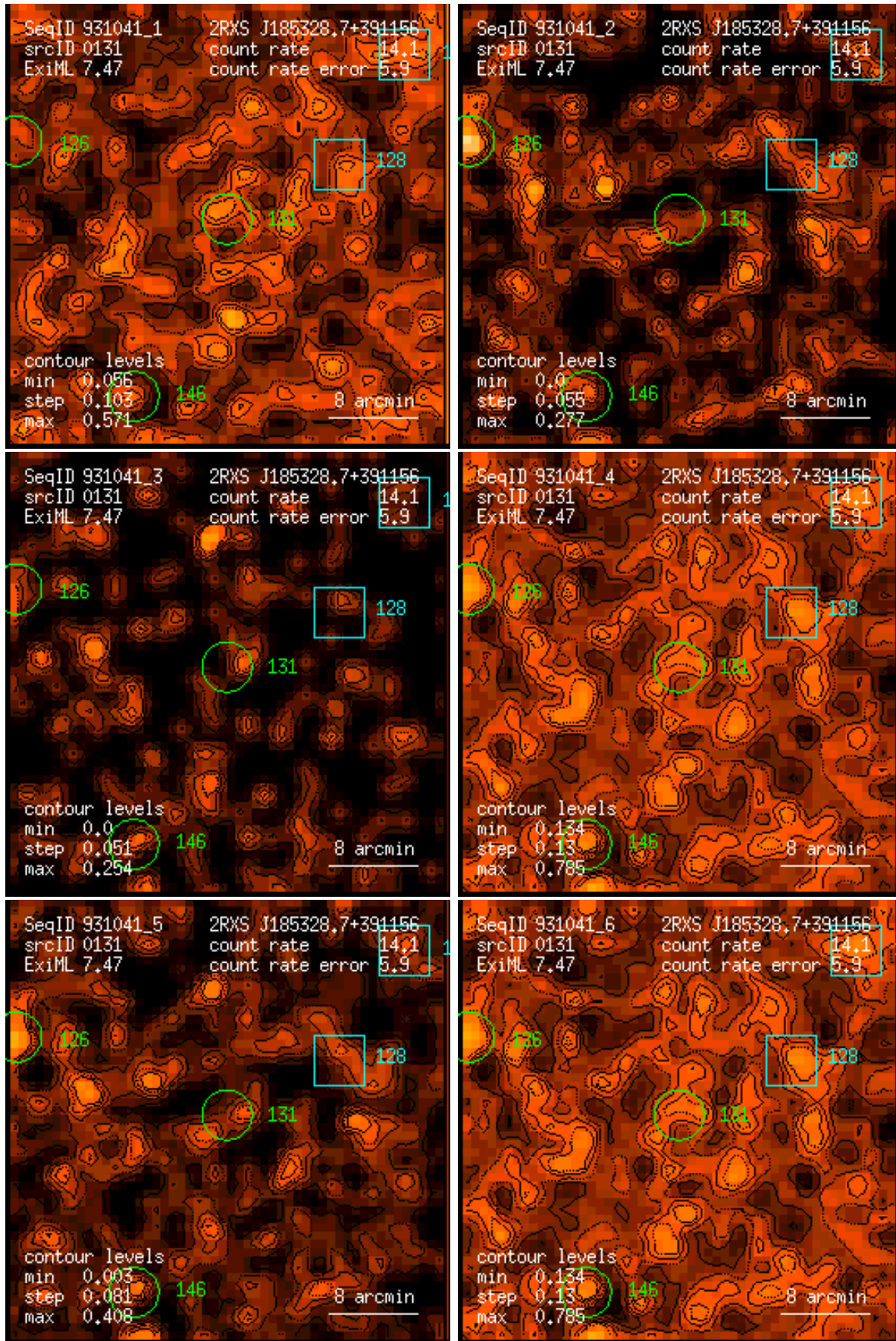
Figure 131: RASS 931041: detection 0131: band rate images, Gaussian filter: (1) PSPC channels 11 – 41, (2) 52 – 90, (3) 91 – 201, (4) 11 – 235, (5) 52 – 201, (6) 11 – 201. Broad band rates in counts/ks. Band rate contour levels in counts/ks/arcmin 2 .
