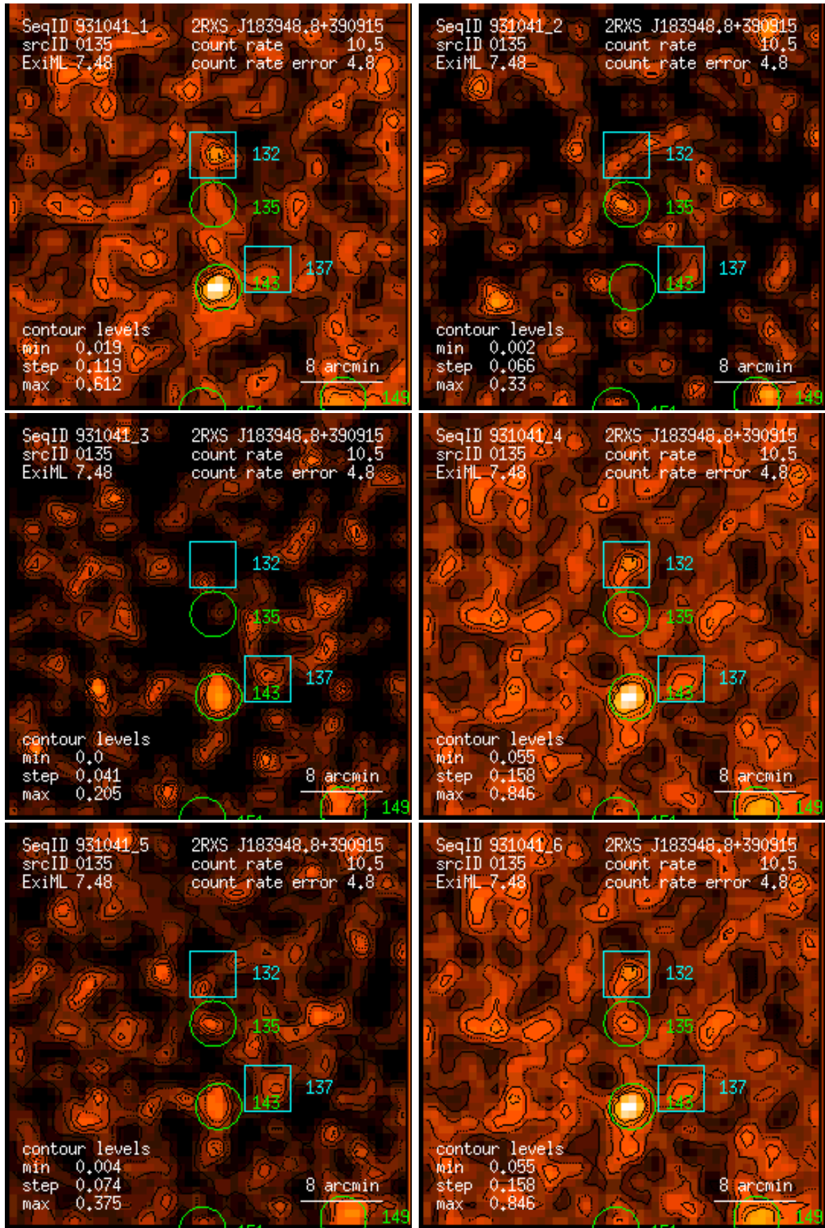
Figure 135: RASS 931041: detection 0135: band rate images, Gaussian filter: (1) PSPC channels 11 – 41, (2) 52 – 90, (3) 91 – 201, (4) 11 – 235, (5) 52 – 201, (6) 11 – 201. Broad band rates in counts/ks. Band rate contour levels in counts/ks/arcmin 2 .
