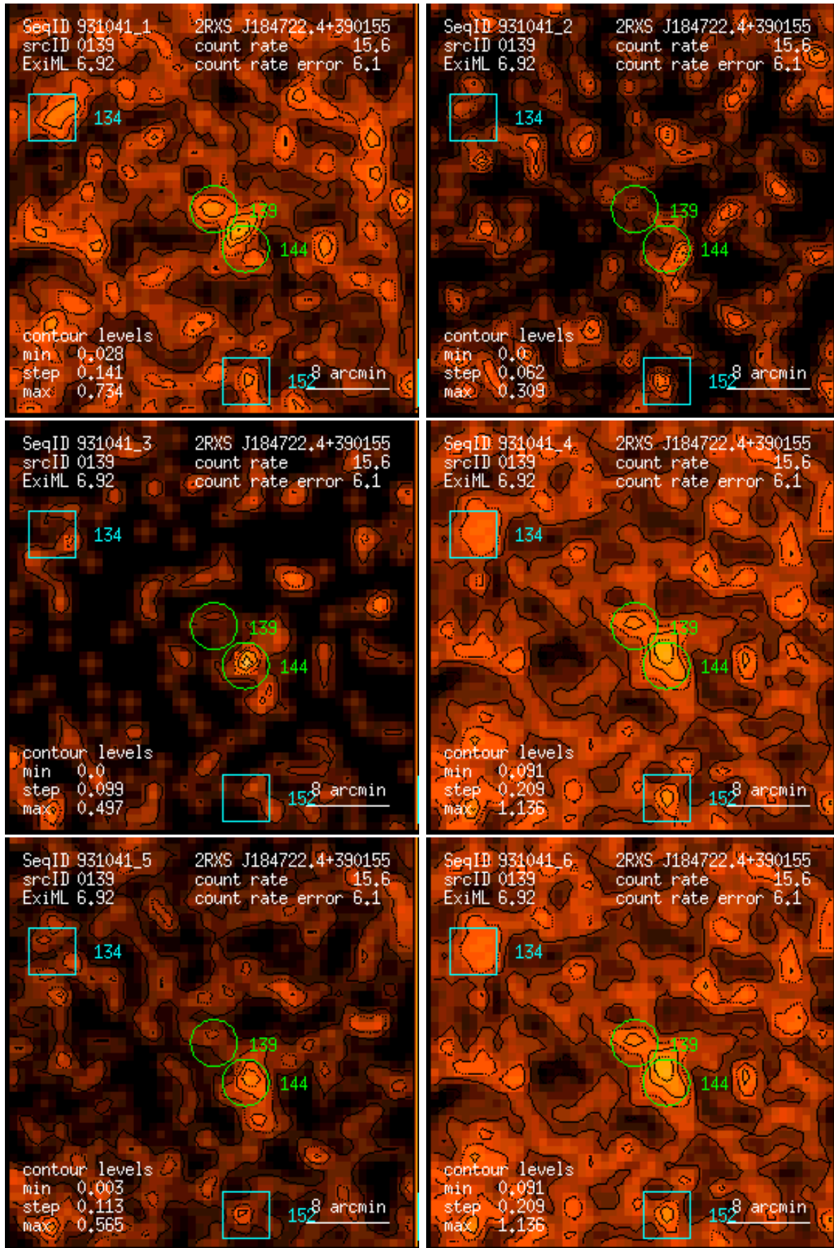
Figure 139: RASS 931041: detection 0139: band rate images, Gaussian filter: (1) PSPC channels 11 – 41, (2) 52 – 90, (3) 91 – 201, (4) 11 – 235, (5) 52 – 201, (6) 11 – 201. Broad band rates in counts/ks. Band rate contour levels in counts/ks/arcmin 2 .
