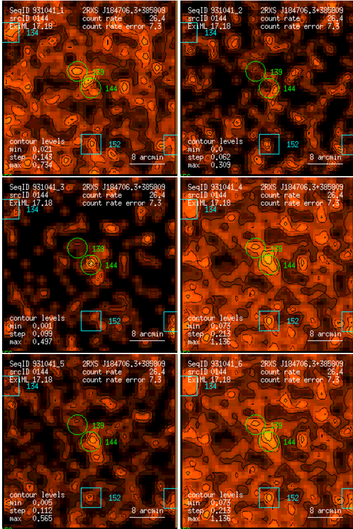
Figure 144: RASS 931041: detection 0144: band rate images, Gaussian filter: (1) PSPC channels 11 – 41, (2) 52 – 90, (3) 91 – 201, (4) 11 – 235, (5) 52 – 201, (6) 11 – 201. Broad band rates in counts/ks. Band rate contour levels in counts/ks/arcmin 2 .
