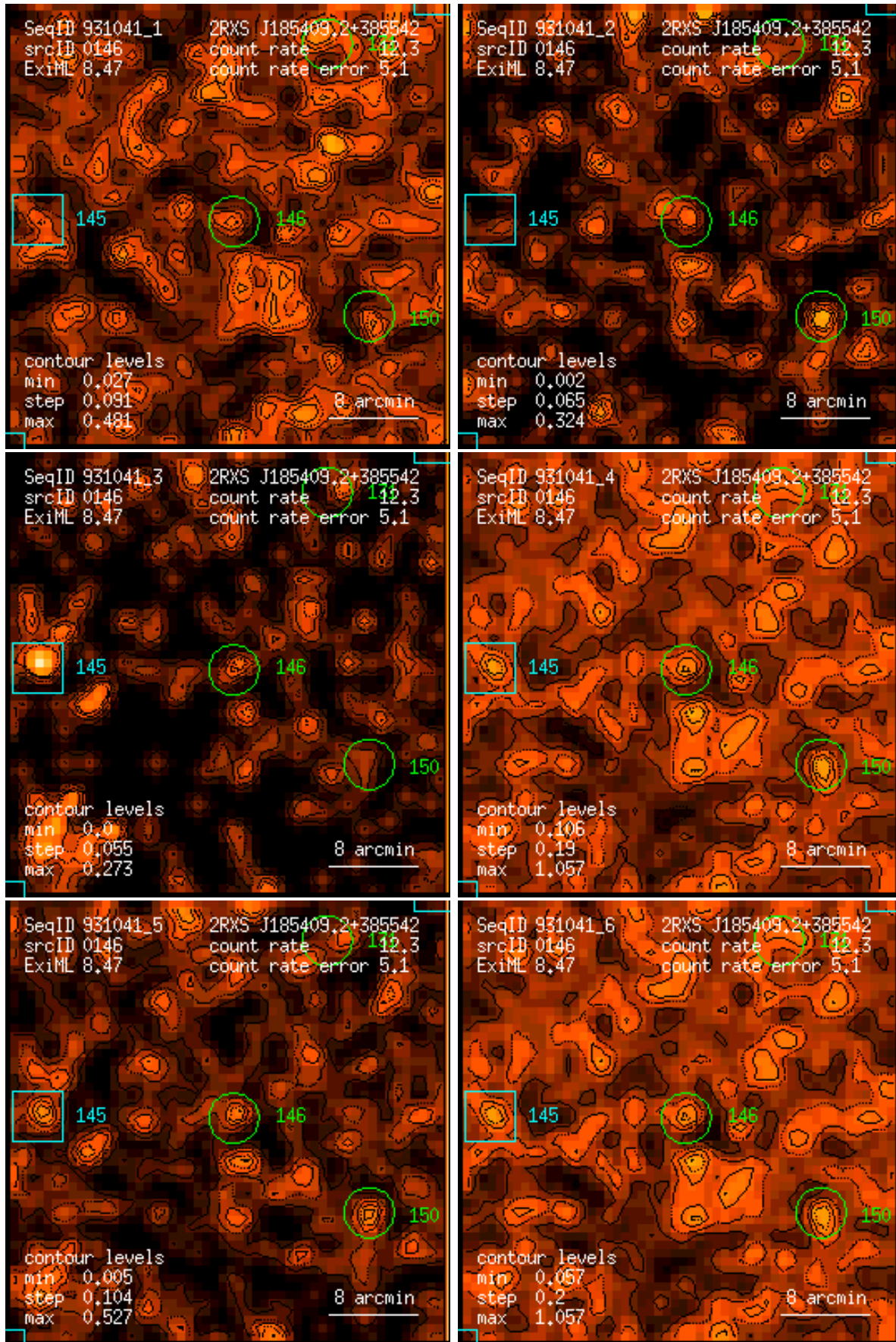
Figure 146: RASS 931041: detection 0146: band rate images, Gaussian filter: (1) PSPC channels 11 – 41, (2) 52 – 90, (3) 91 – 201, (4) 11 – 235, (5) 52 – 201, (6) 11 – 201. Broad band rates in counts/ks. Band rate contour levels in counts/ks/arcmin 2 .
