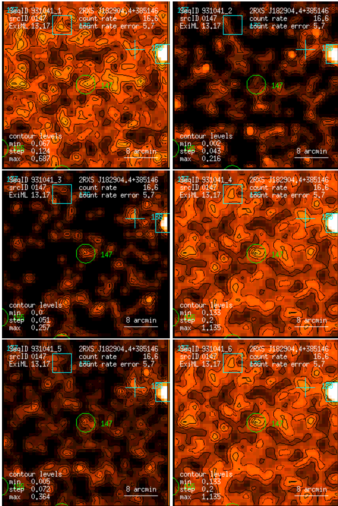
Figure 147: RASS 931041: detection 0147: band rate images, Gaussian filter: (1) PSPC channels 11 – 41, (2) 52 – 90, (3) 91 – 201, (4) 11 – 235, (5) 52 – 201, (6) 11 – 201. Broad band rates in counts/ks. Band rate contour levels in counts/ks/arcmin 2 .
