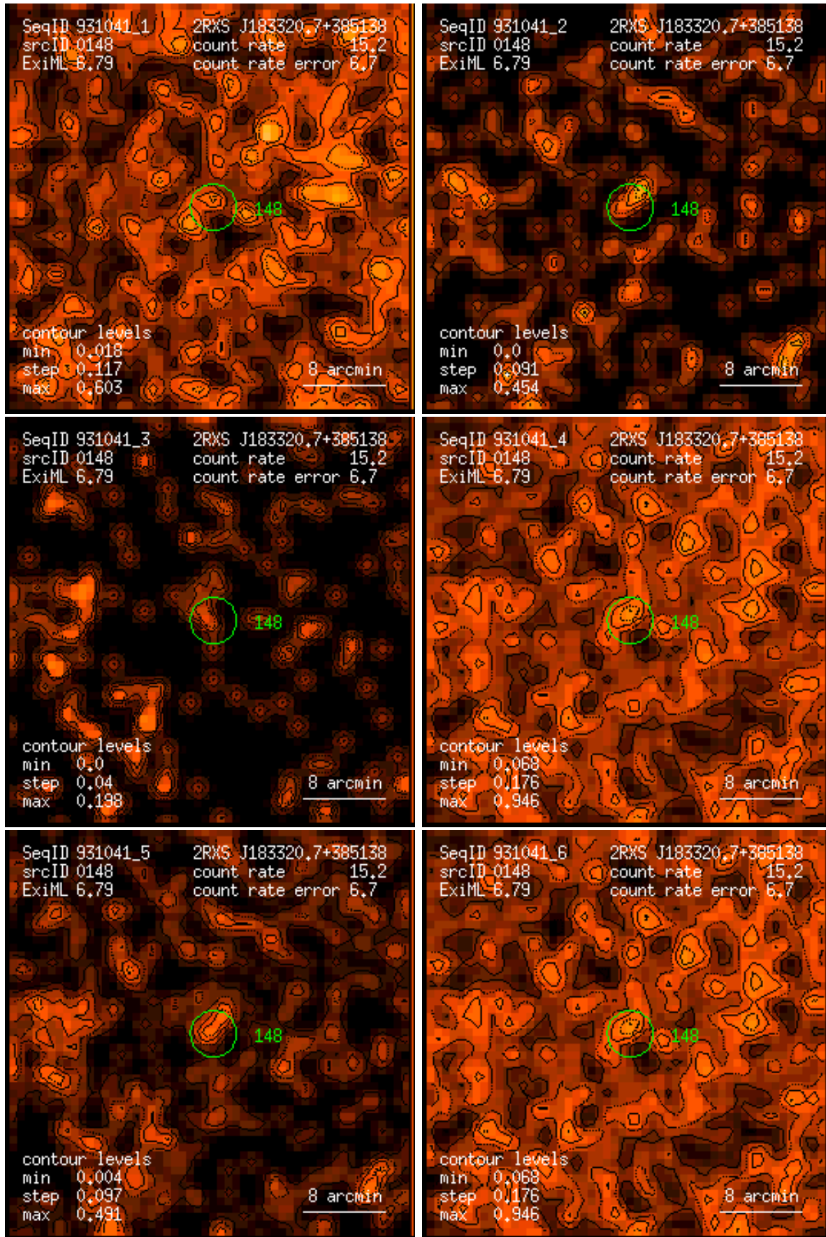
Figure 148: RASS 931041: detection 0148: band rate images, Gaussian filter: (1) PSPC channels 11 – 41, (2) 52 – 90, (3) 91 – 201, (4) 11 – 235, (5) 52 – 201, (6) 11 – 201. Broad band rates in counts/ks. Band rate contour levels in counts/ks/arcmin 2 .
