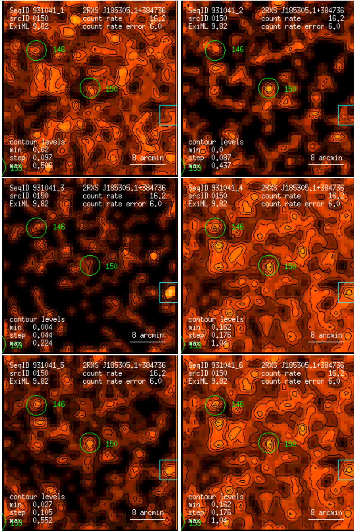
Figure 150: RASS 931041: detection 0150: band rate images, Gaussian filter: (1) PSPC channels 11 – 41, (2) 52 – 90, (3) 91 – 201, (4) 11 – 235, (5) 52 – 201, (6) 11 – 201. Broad band rates in counts/ks. Band rate contour levels in counts/ks/arcmin 2 .
