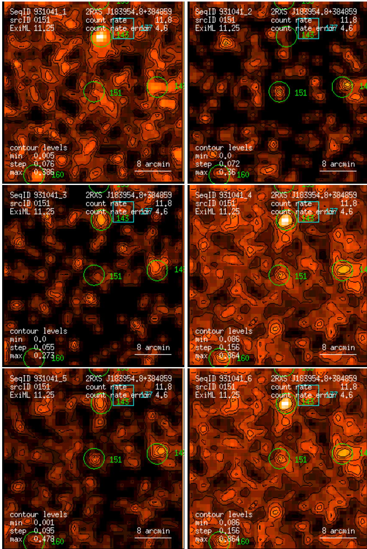
Figure 151: RASS 931041: detection 0151: band rate images, Gaussian filter: (1) PSPC channels 11 – 41, (2) 52 – 90, (3) 91 – 201, (4) 11 – 235, (5) 52 – 201, (6) 11 – 201. Broad band rates in counts/ks. Band rate contour levels in counts/ks/arcmin 2 .
