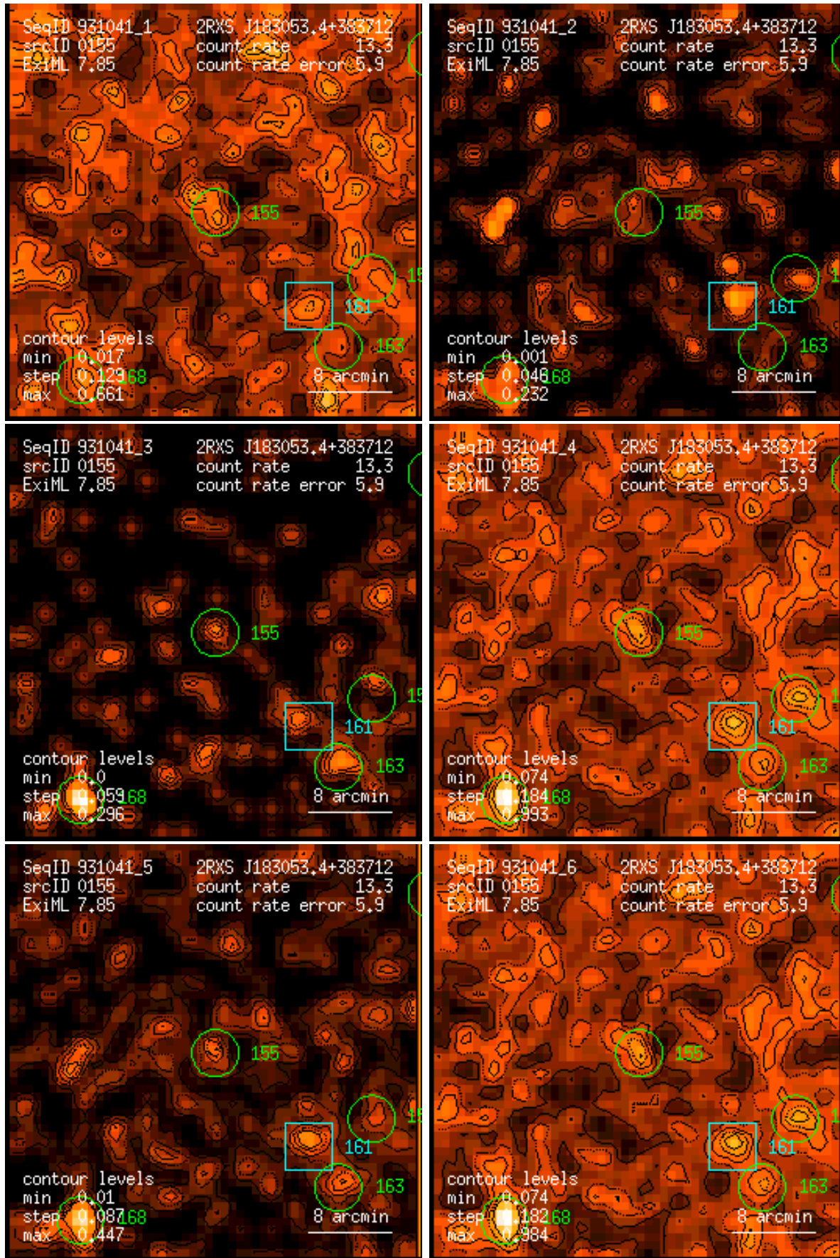
Figure 155: RASS 931041: detection 0155: band rate images, Gaussian filter: (1) PSPC channels 11 – 41, (2) 52 – 90, (3) 91 – 201, (4) 11 – 235, (5) 52 – 201, (6) 11 – 201. Broad band rates in counts/ks. Band rate contour levels in counts/ks/arcmin 2 .
