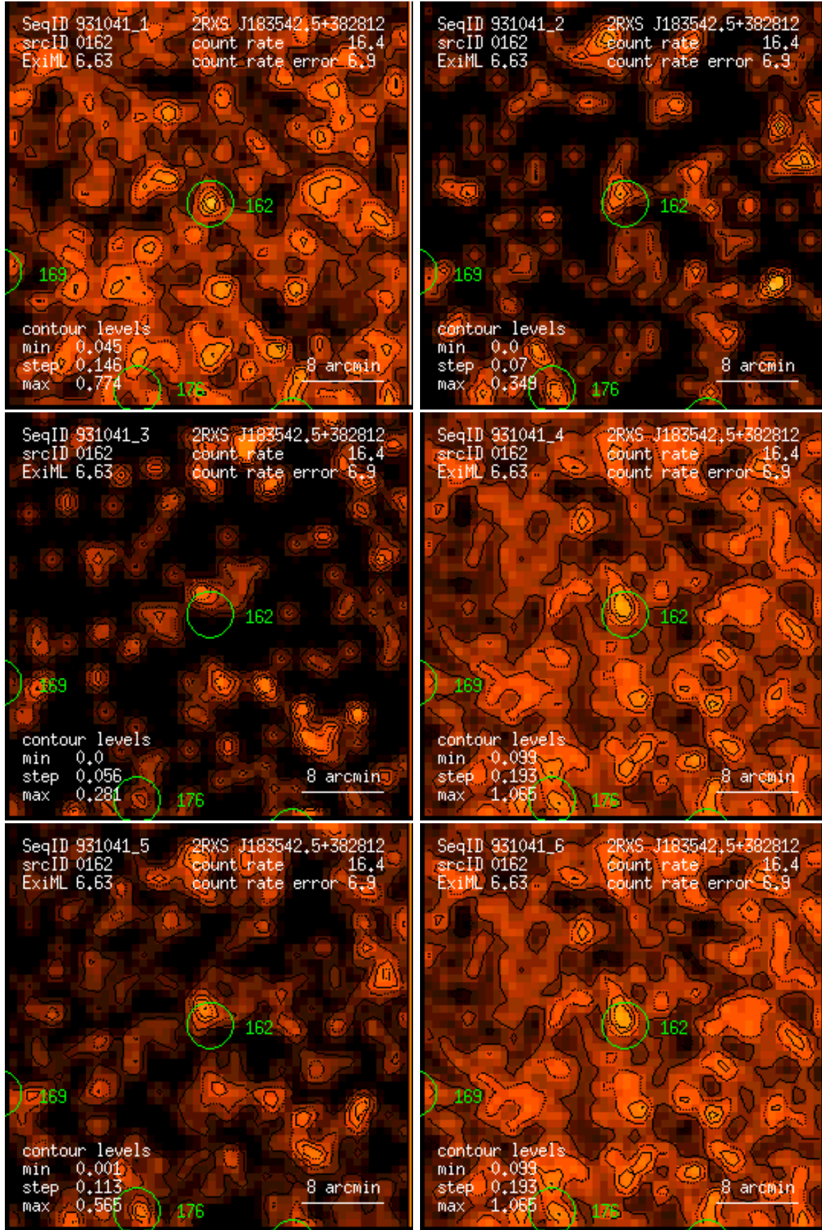
Figure 162: RASS 931041: detection 0162: band rate images, Gaussian filter: (1) PSPC channels 11 – 41, (2) 52 – 90, (3) 91 – 201, (4) 11 – 235, (5) 52 – 201, (6) 11 – 201. Broad band rates in counts/ks. Band rate contour levels in counts/ks/arcmin 2 .
