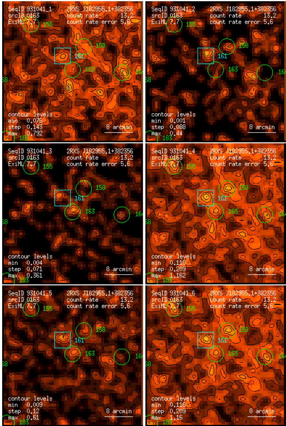
Figure 163: RASS 931041: detection 0163: band rate images, Gaussian filter: (1) PSPC channels 11 – 41, (2) 52 – 90, (3) 91 – 201, (4) 11 – 235, (5) 52 – 201, (6) 11 – 201. Broad band rates in counts/ks. Band rate contour levels in counts/ks/arcmin 2 .
