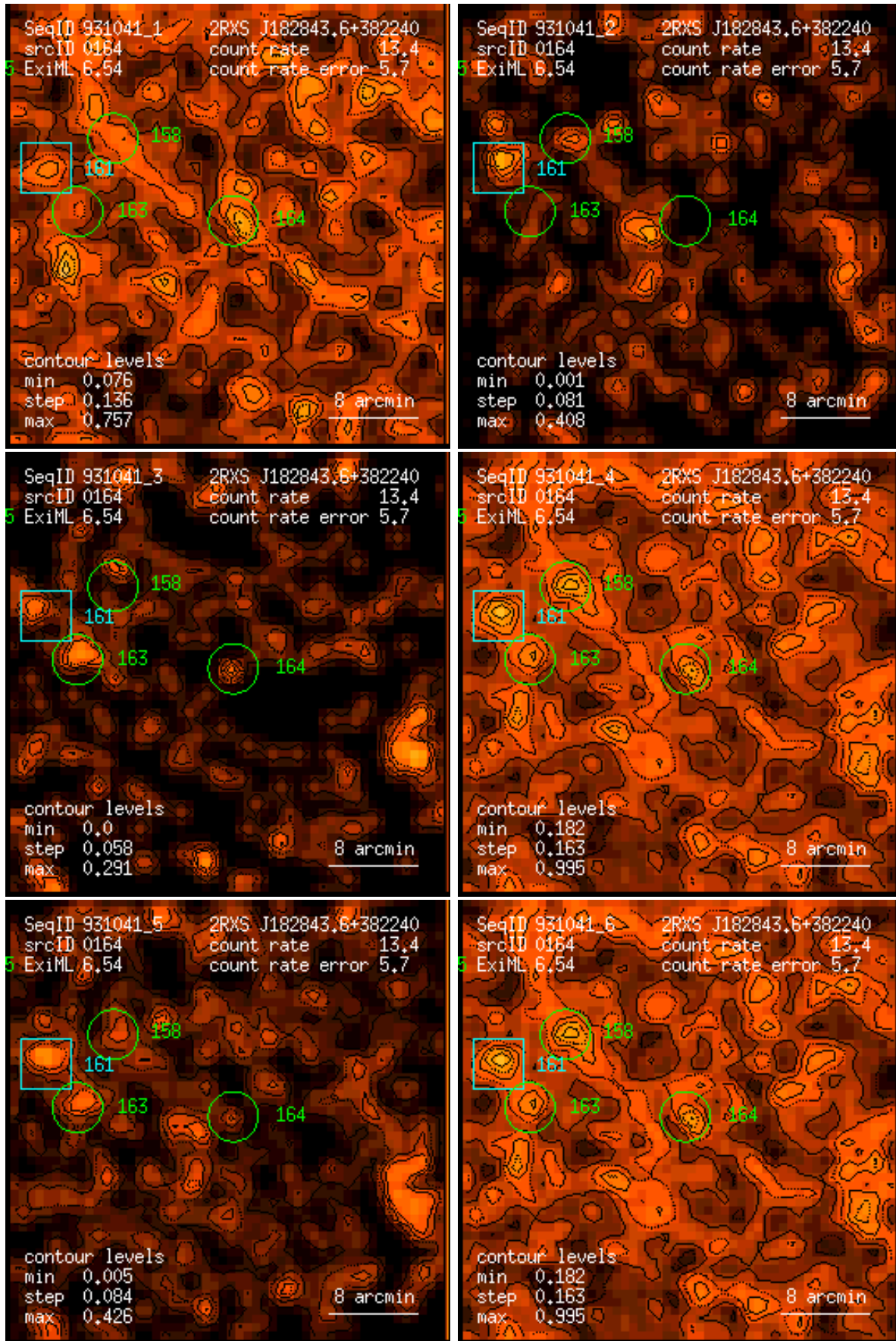
Figure 164: RASS 931041: detection 0164: band rate images, Gaussian filter: (1) PSPC channels 11 – 41, (2) 52 – 90, (3) 91 – 201, (4) 11 – 235, (5) 52 – 201, (6) 11 – 201. Broad band rates in counts/ks. Band rate contour levels in counts/ks/arcmin 2 .
