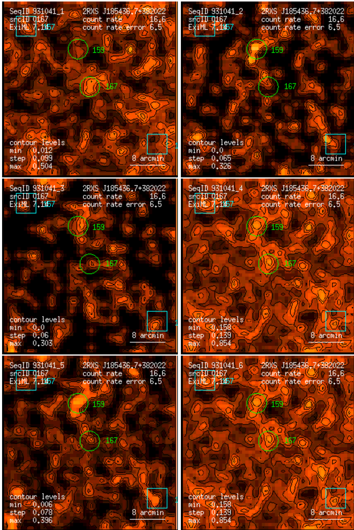
Figure 167: RASS 931041: detection 0167: band rate images, Gaussian filter: (1) PSPC channels 11 – 41, (2) 52 – 90, (3) 91 – 201, (4) 11 – 235, (5) 52 – 201, (6) 11 – 201. Broad band rates in counts/ks. Band rate contour levels in counts/ks/arcmin 2 .
