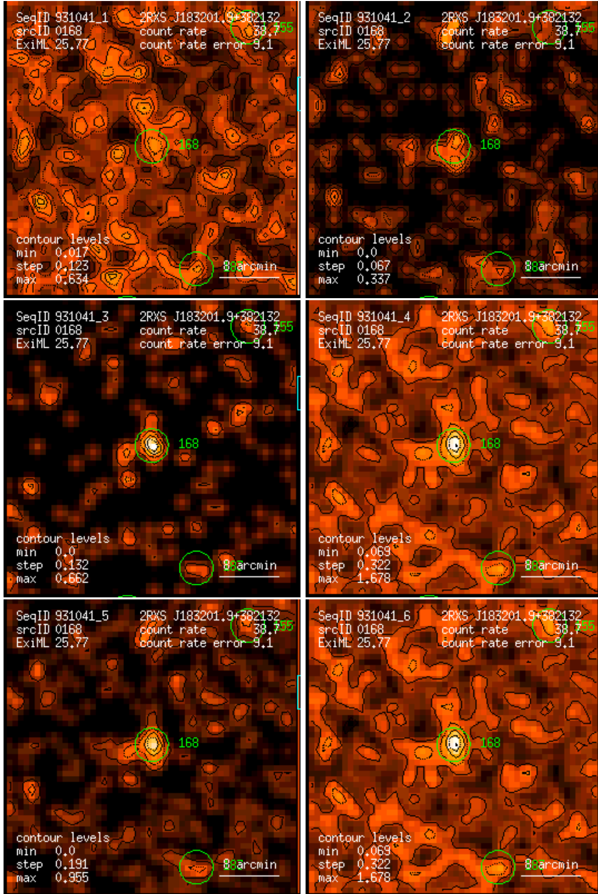
Figure 168: RASS 931041: detection 0168: band rate images, Gaussian filter: (1) PSPC channels 11 – 41, (2) 52 – 90, (3) 91 – 201, (4) 11 – 235, (5) 52 – 201, (6) 11 – 201. Broad band rates in counts/ks. Band rate contour levels in counts/ks/arcmin 2 .
