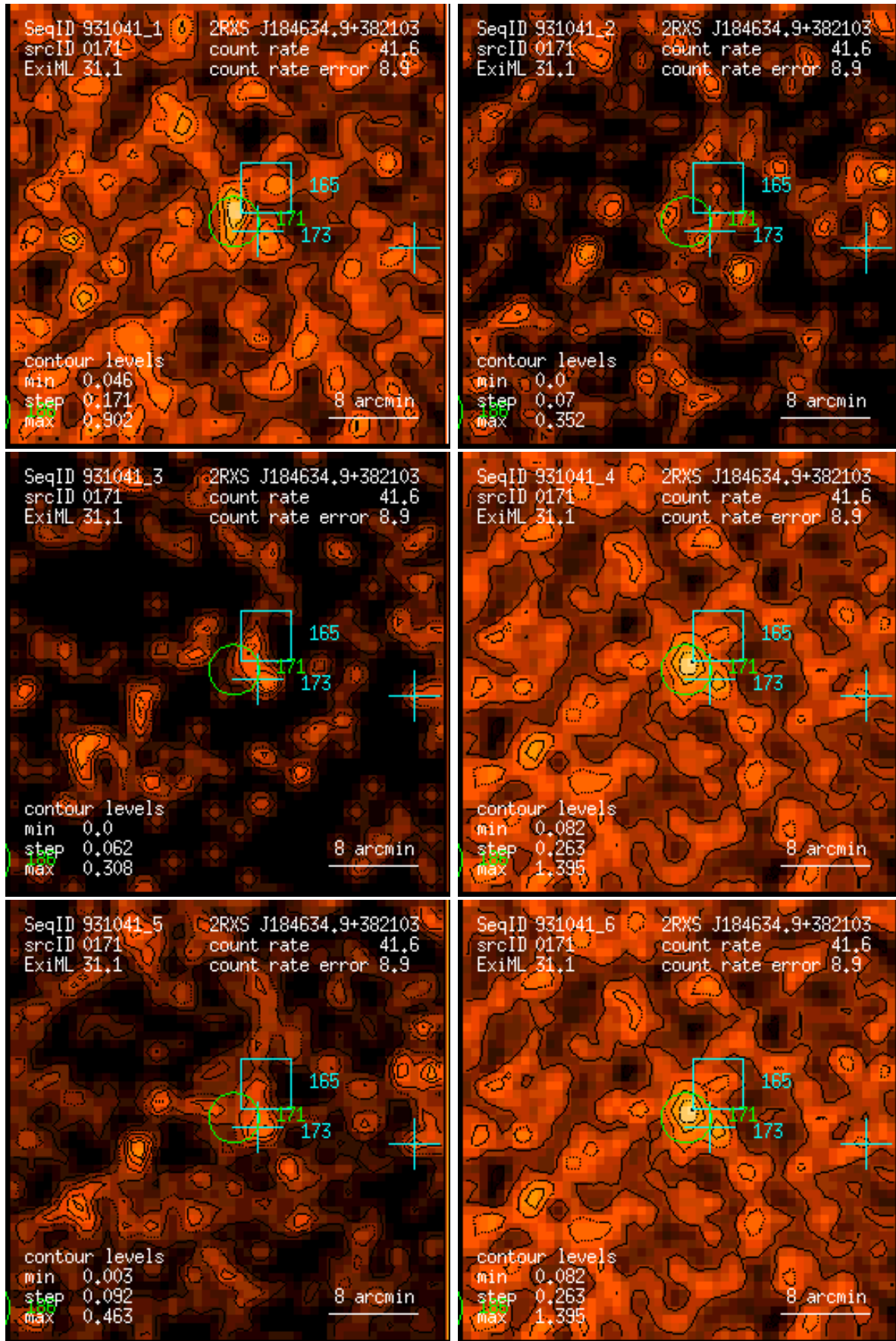
Figure 171: RASS 931041: detection 0171: band rate images, Gaussian filter: (1) PSPC channels 11 – 41, (2) 52 – 90, (3) 91 – 201, (4) 11 – 235, (5) 52 – 201, (6) 11 – 201. Broad band rates in counts/ks. Band rate contour levels in counts/ks/arcmin 2 .
