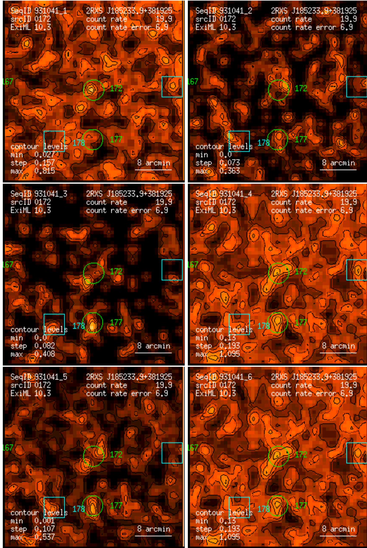
Figure 172: RASS 931041: detection 0172: band rate images, Gaussian filter: (1) PSPC channels 11 – 41, (2) 52 – 90, (3) 91 – 201, (4) 11 – 235, (5) 52 – 201, (6) 11 – 201. Broad band rates in counts/ks. Band rate contour levels in counts/ks/arcmin 2 .
