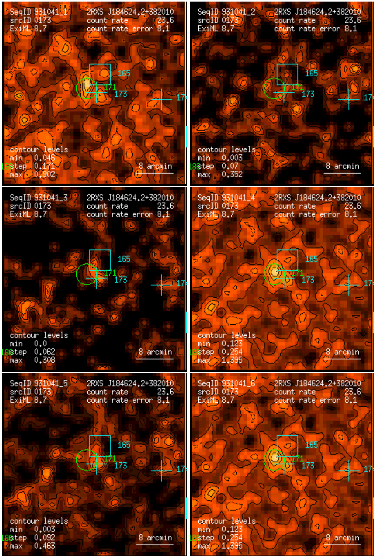
Figure 173: RASS 931041: detection 0173: band rate images, Gaussian filter: (1) PSPC channels 11 – 41, (2) 52 – 90, (3) 91 – 201, (4) 11 – 235, (5) 52 – 201, (6) 11 – 201. Broad band rates in counts/ks. Band rate contour levels in counts/ks/arcmin 2 .
