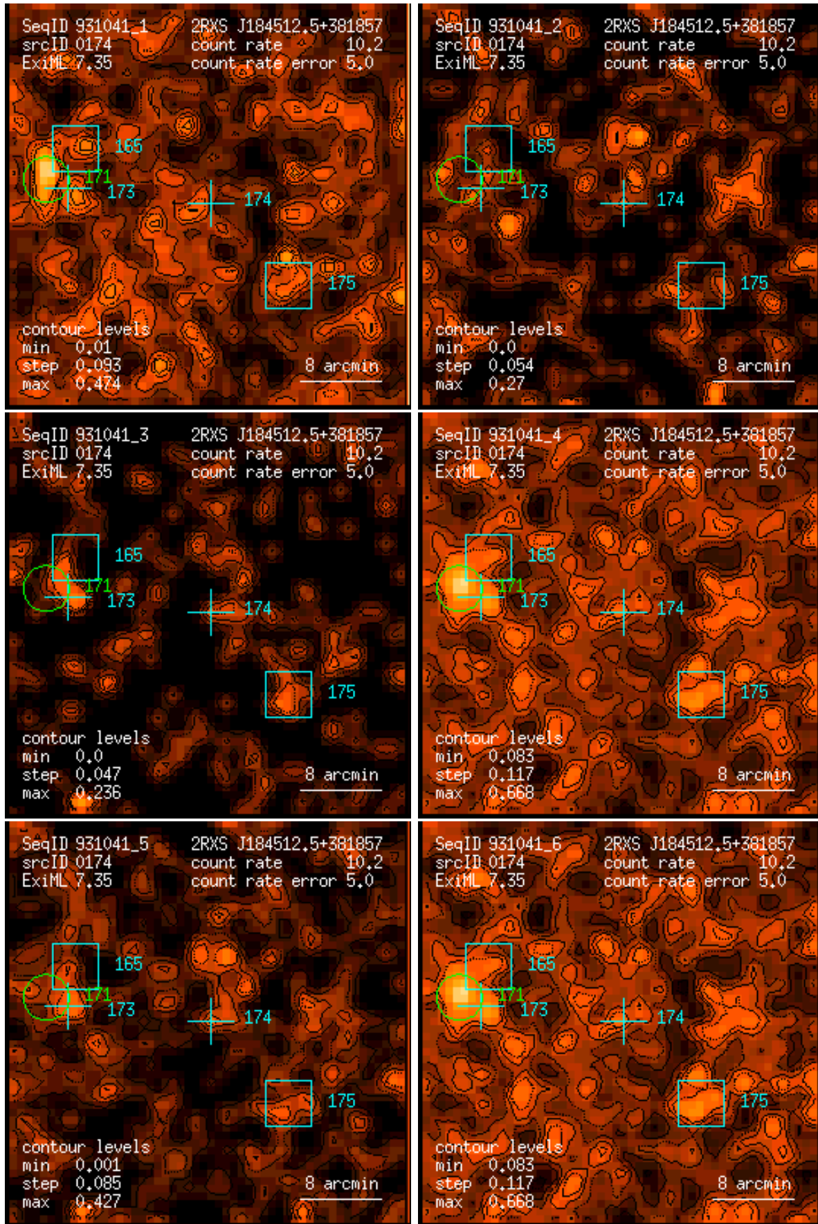
Figure 174: RASS 931041: detection 0174: band rate images, Gaussian filter: (1) PSPC channels 11 – 41, (2) 52 – 90, (3) 91 – 201, (4) 11 – 235, (5) 52 – 201, (6) 11 – 201. Broad band rates in counts/ks. Band rate contour levels in counts/ks/arcmin 2 .
