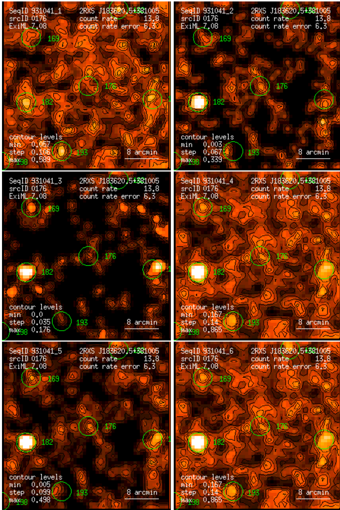
Figure 176: RASS 931041: detection 0176: band rate images, Gaussian filter: (1) PSPC channels 11 – 41, (2) 52 – 90, (3) 91 – 201, (4) 11 – 235, (5) 52 – 201, (6) 11 – 201. Broad band rates in counts/ks. Band rate contour levels in counts/ks/arcmin 2 .
