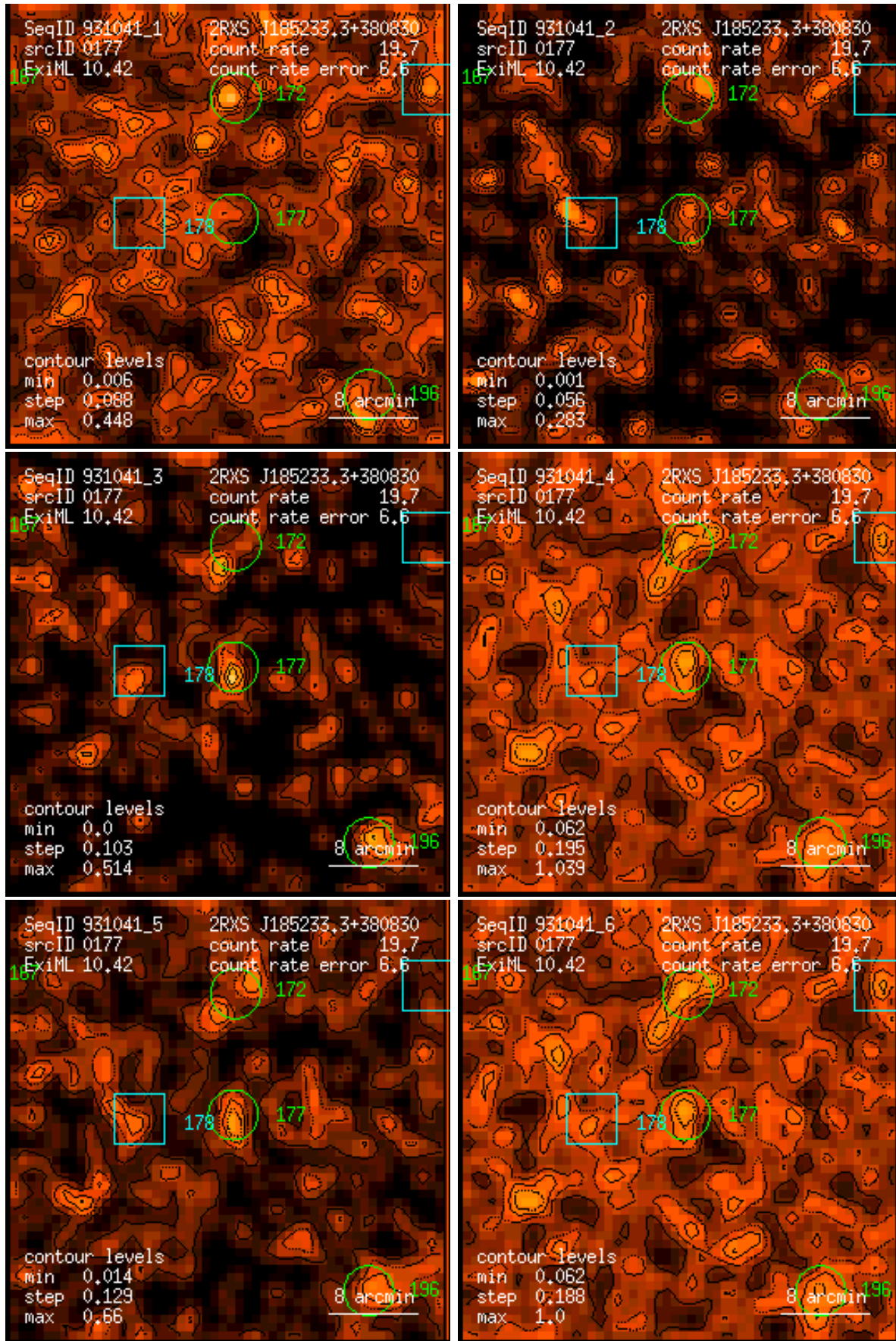
Figure 177: RASS 931041: detection 0177: band rate images, Gaussian filter: (1) PSPC channels 11 – 41, (2) 52 – 90, (3) 91 – 201, (4) 11 – 235, (5) 52 – 201, (6) 11 – 201. Broad band rates in counts/ks. Band rate contour levels in counts/ks/arcmin 2 .
