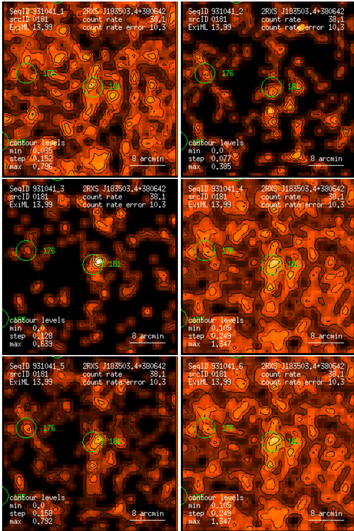
Figure 181: RASS 931041: detection 0181: band rate images, Gaussian filter: (1) PSPC channels 11 – 41, (2) 52 – 90, (3) 91 – 201, (4) 11 – 235, (5) 52 – 201, (6) 11 – 201. Broad band rates in counts/ks. Band rate contour levels in counts/ks/arcmin 2 .
