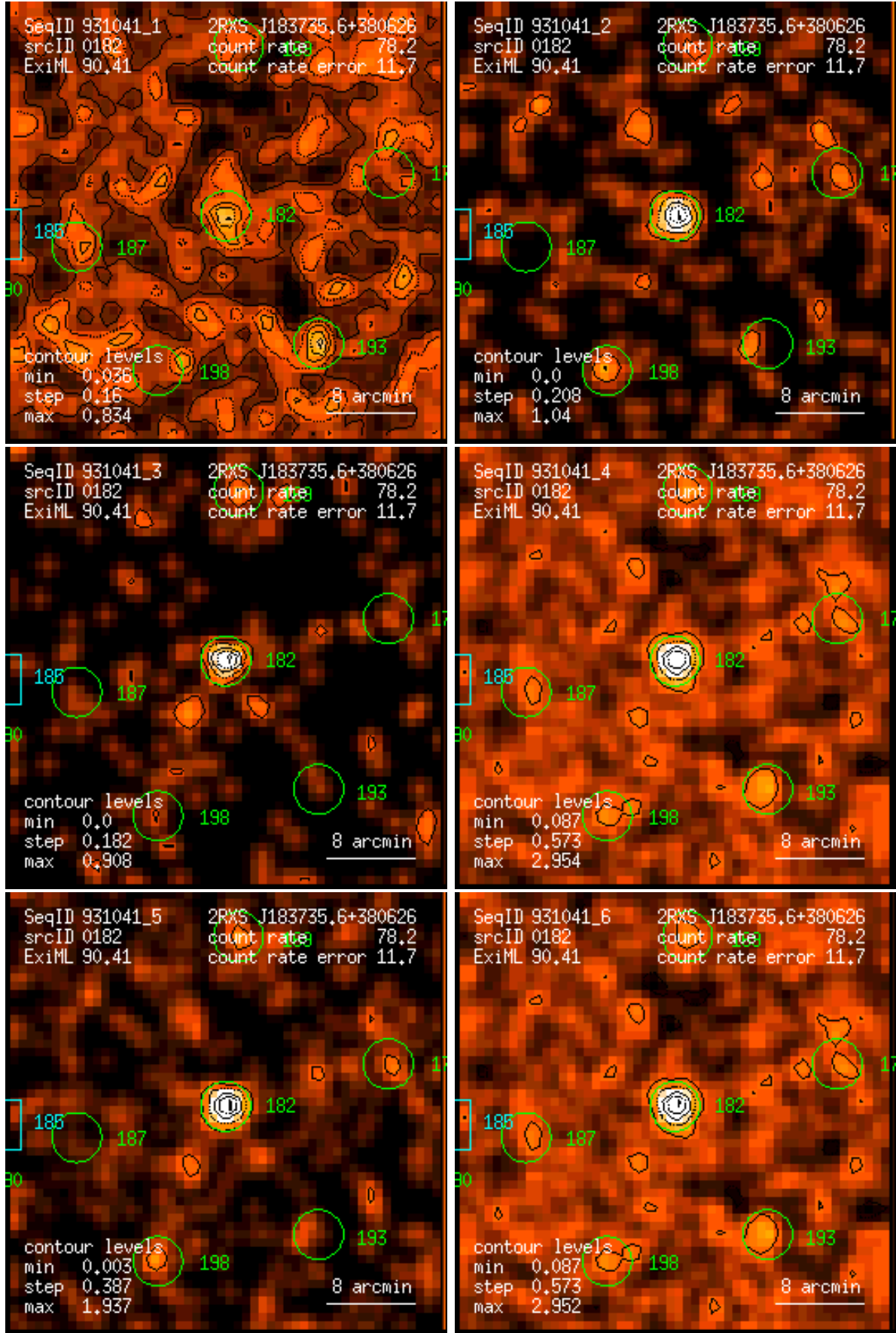
Figure 182: RASS 931041: detection 0182: band rate images, Gaussian filter: (1) PSPC channels 11 – 41, (2) 52 – 90, (3) 91 – 201, (4) 11 – 235, (5) 52 – 201, (6) 11 – 201. Broad band rates in counts/ks. Band rate contour levels in counts/ks/arcmin 2 .
