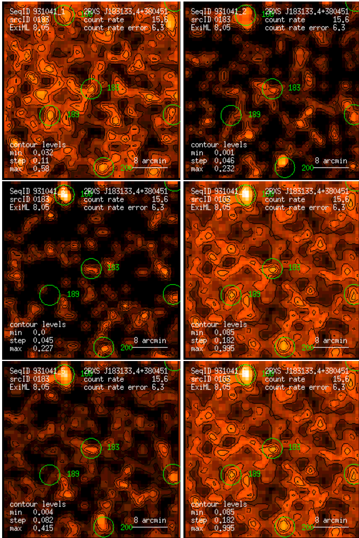
Figure 183: RASS 931041: detection 0183: band rate images, Gaussian filter: (1) PSPC channels 11 – 41, (2) 52 – 90, (3) 91 – 201, (4) 11 – 235, (5) 52 – 201, (6) 11 – 201. Broad band rates in counts/ks. Band rate contour levels in counts/ks/arcmin 2 .
