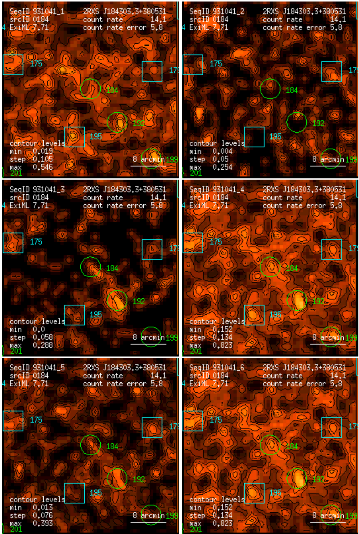
Figure 184: RASS 931041: detection 0184: band rate images, Gaussian filter: (1) PSPC channels 11 – 41, (2) 52 – 90, (3) 91 – 201, (4) 11 – 235, (5) 52 – 201, (6) 11 – 201. Broad band rates in counts/ks. Band rate contour levels in counts/ks/arcmin 2 .
