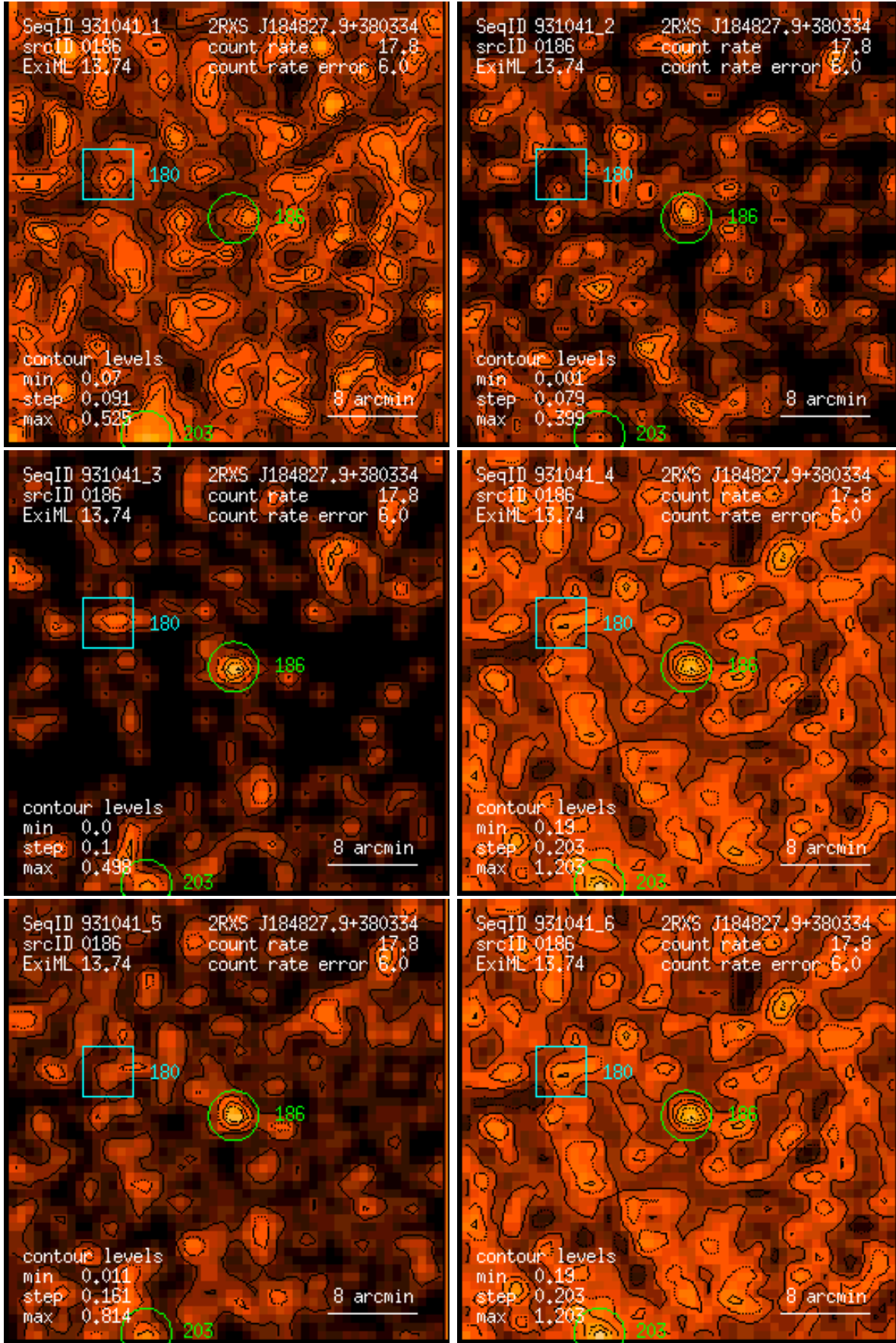
Figure 186: RASS 931041: detection 0186: band rate images, Gaussian filter: (1) PSPC channels 11 – 41, (2) 52 – 90, (3) 91 – 201, (4) 11 – 235, (5) 52 – 201, (6) 11 – 201. Broad band rates in counts/ks. Band rate contour levels in counts/ks/arcmin 2 .
