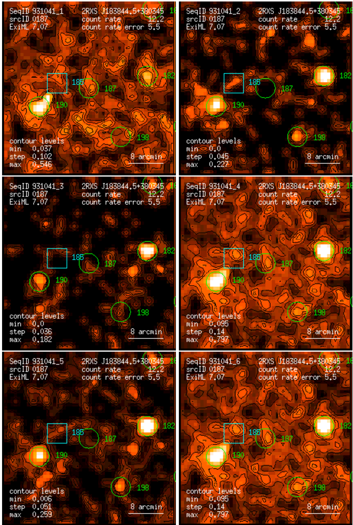
Figure 187: RASS 931041: detection 0187: band rate images, Gaussian filter: (1) PSPC channels 11 – 41, (2) 52 – 90, (3) 91 – 201, (4) 11 – 235, (5) 52 – 201, (6) 11 – 201. Broad band rates in counts/ks. Band rate contour levels in counts/ks/arcmin 2 .
