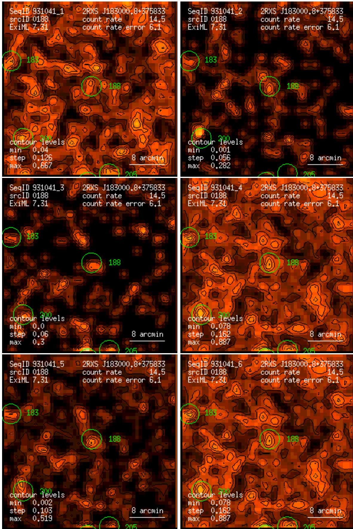
Figure 188: RASS 931041: detection 0188: band rate images, Gaussian filter: (1) PSPC channels 11 – 41, (2) 52 – 90, (3) 91 – 201, (4) 11 – 235, (5) 52 – 201, (6) 11 – 201. Broad band rates in counts/ks. Band rate contour levels in counts/ks/arcmin 2 .
