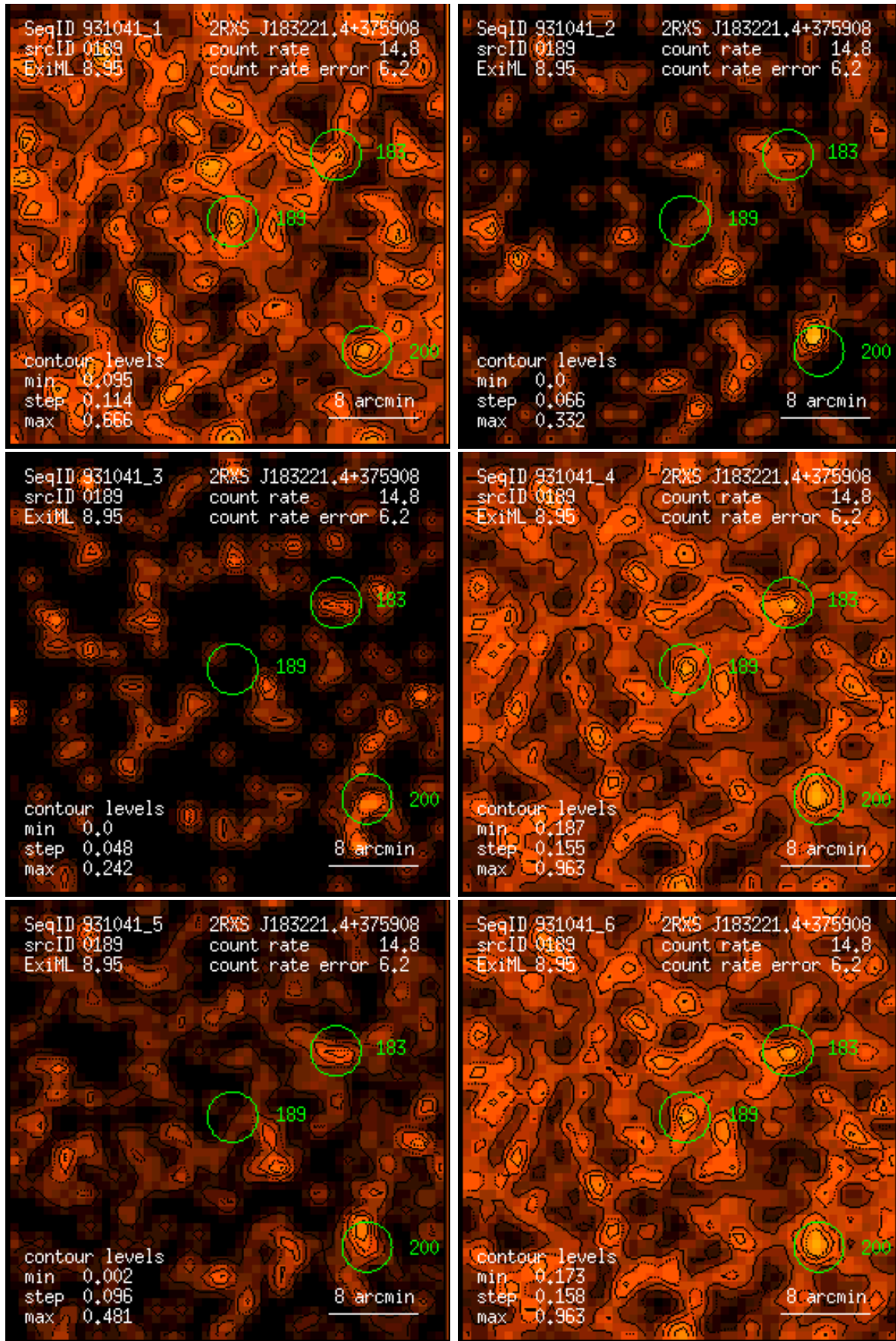
Figure 189: RASS 931041: detection 0189: band rate images, Gaussian filter: (1) PSPC channels 11 – 41, (2) 52 – 90, (3) 91 – 201, (4) 11 – 235, (5) 52 – 201, (6) 11 – 201. Broad band rates in counts/ks. Band rate contour levels in counts/ks/arcmin 2 .
