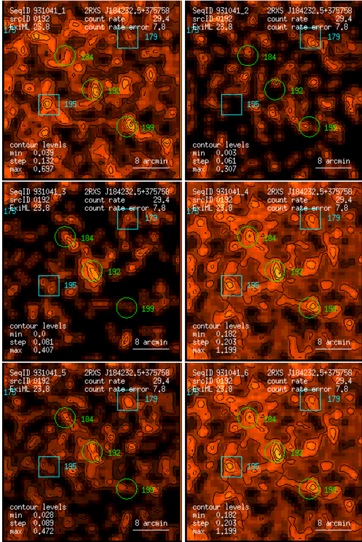
Figure 192: RASS 931041: detection 0192: band rate images, Gaussian filter: (1) PSPC channels 11 – 41, (2) 52 – 90, (3) 91 – 201, (4) 11 – 235, (5) 52 – 201, (6) 11 – 201. Broad band rates in counts/ks. Band rate contour levels in counts/ks/arcmin 2 .
