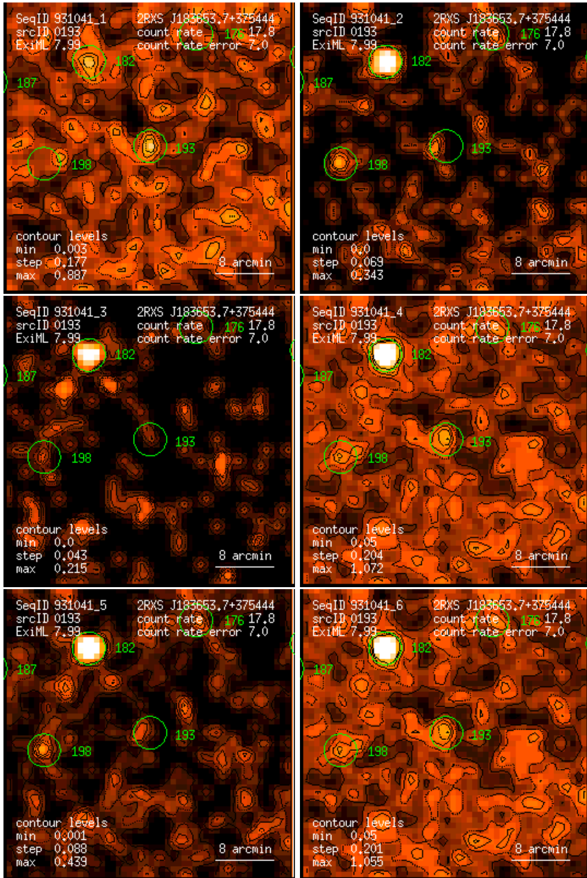
Figure 193: RASS 931041: detection 0193: band rate images, Gaussian filter: (1) PSPC channels 11 – 41, (2) 52 – 90, (3) 91 – 201, (4) 11 – 235, (5) 52 – 201, (6) 11 – 201. Broad band rates in counts/ks. Band rate contour levels in counts/ks/arcmin 2 .
