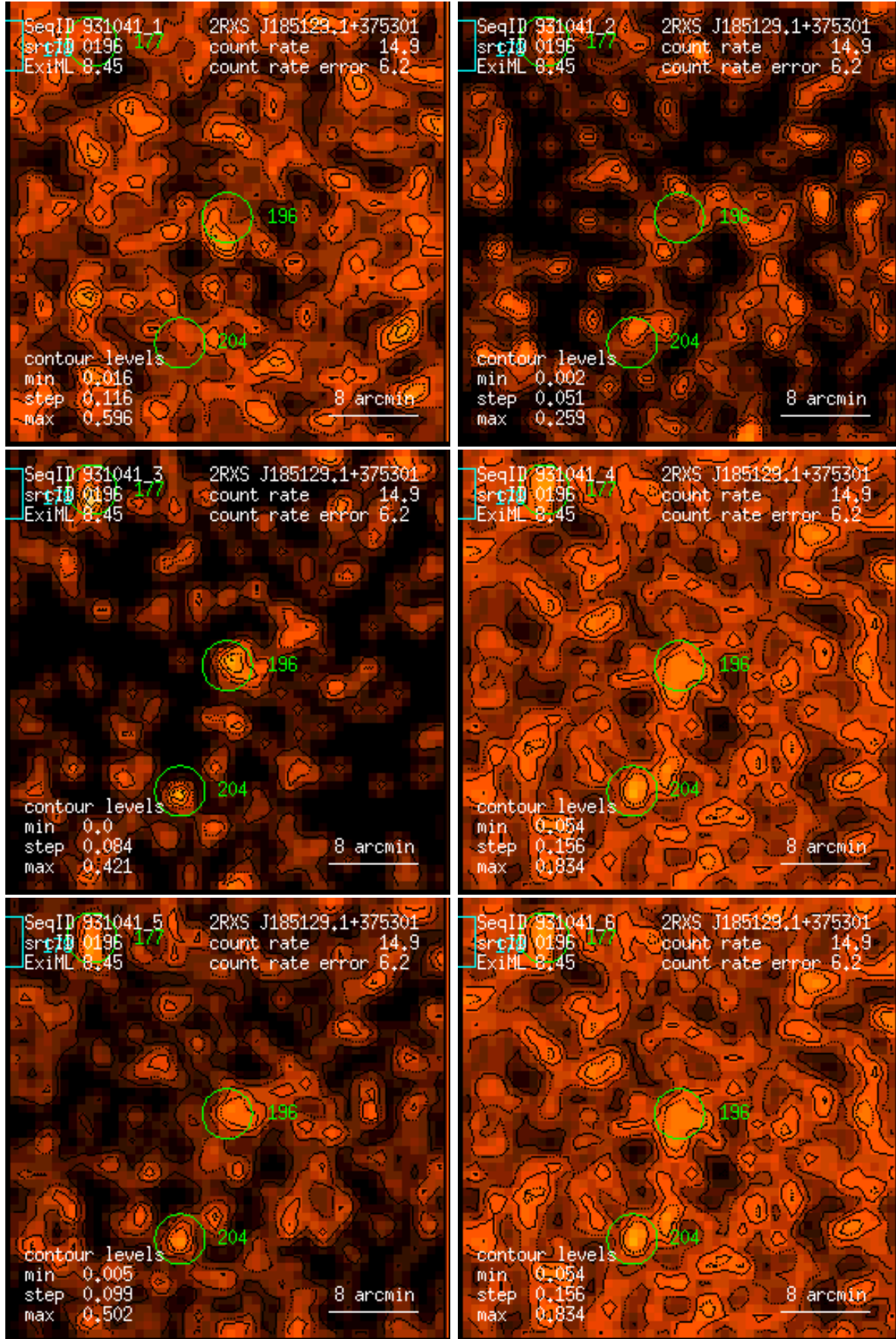
Figure 196: RASS 931041: detection 0196: band rate images, Gaussian filter: (1) PSPC channels 11 – 41, (2) 52 – 90, (3) 91 – 201, (4) 11 – 235, (5) 52 – 201, (6) 11 – 201. Broad band rates in counts/ks. Band rate contour levels in counts/ks/arcmin 2 .
