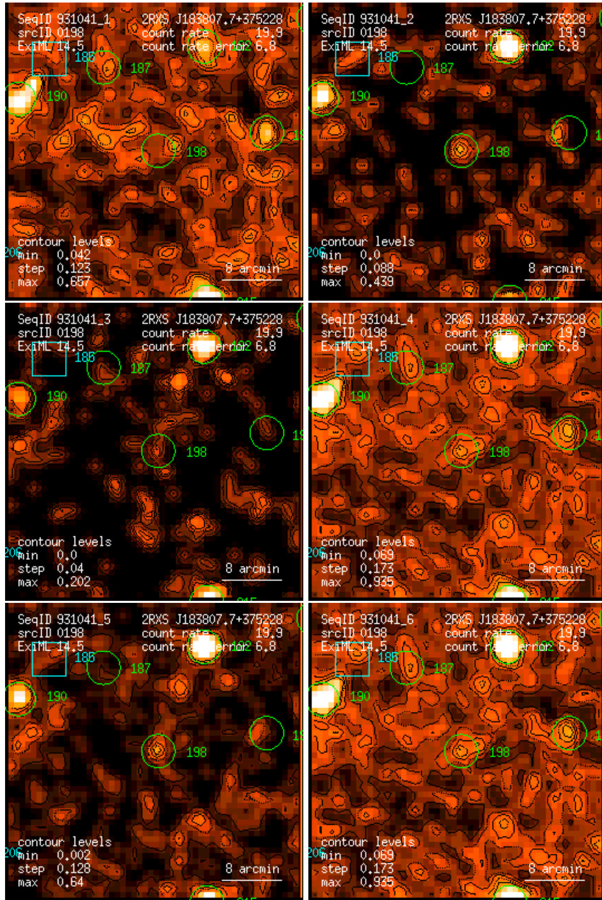
Figure 198: RASS 931041: detection 0198: band rate images, Gaussian filter: (1) PSPC channels 11 – 41, (2) 52 – 90, (3) 91 – 201, (4) 11 – 235, (5) 52 – 201, (6) 11 – 201. Broad band rates in counts/ks. Band rate contour levels in counts/ks/arcmin 2 .
