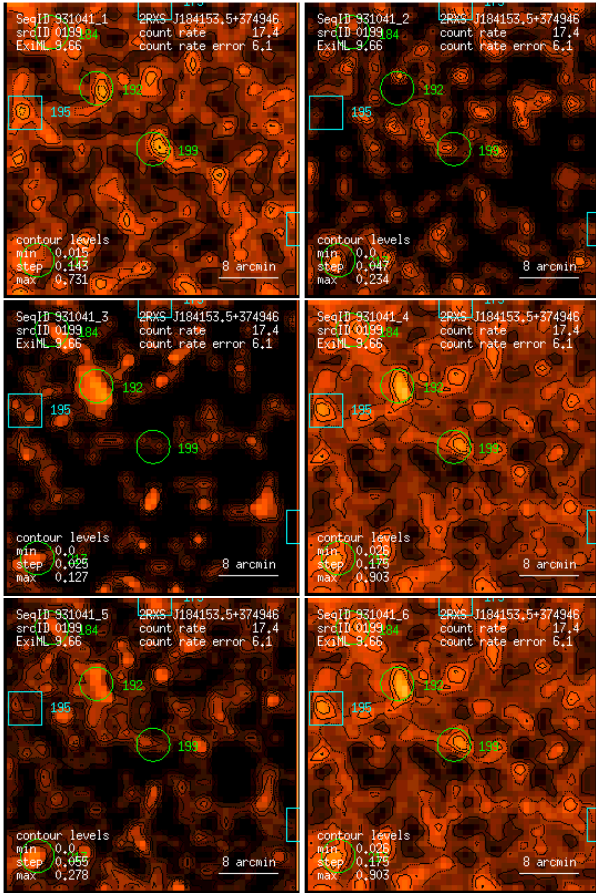
Figure 199: RASS 931041: detection 0199: band rate images, Gaussian filter: (1) PSPC channels 11 – 41, (2) 52 – 90, (3) 91 – 201, (4) 11 – 235, (5) 52 – 201, (6) 11 – 201. Broad band rates in counts/ks. Band rate contour levels in counts/ks/arcmin 2 .
