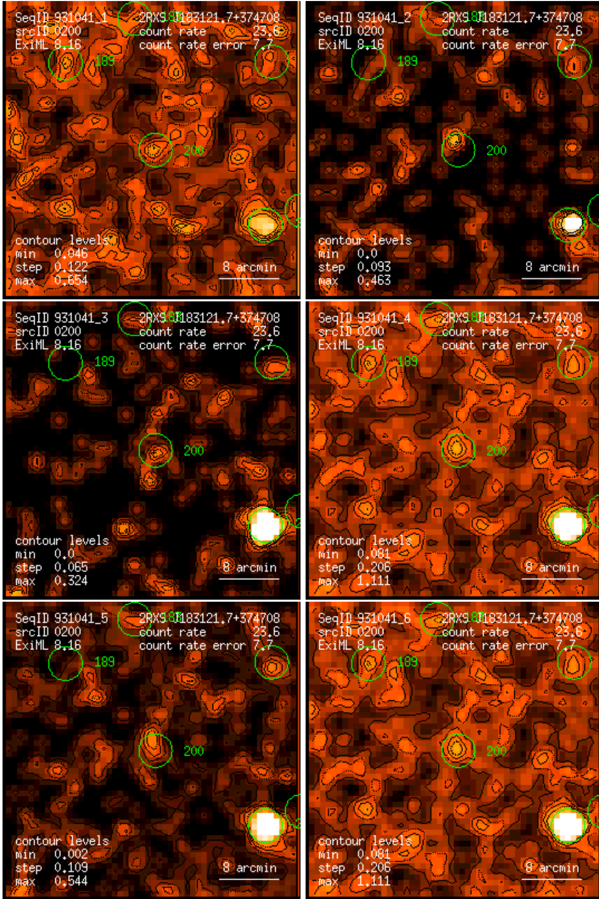
Figure 200: RASS 931041: detection 0200: band rate images, Gaussian filter: (1) PSPC channels 11 – 41, (2) 52 – 90, (3) 91 – 201, (4) 11 – 235, (5) 52 – 201, (6) 11 – 201. Broad band rates in counts/ks. Band rate contour levels in counts/ks/arcmin 2 .
