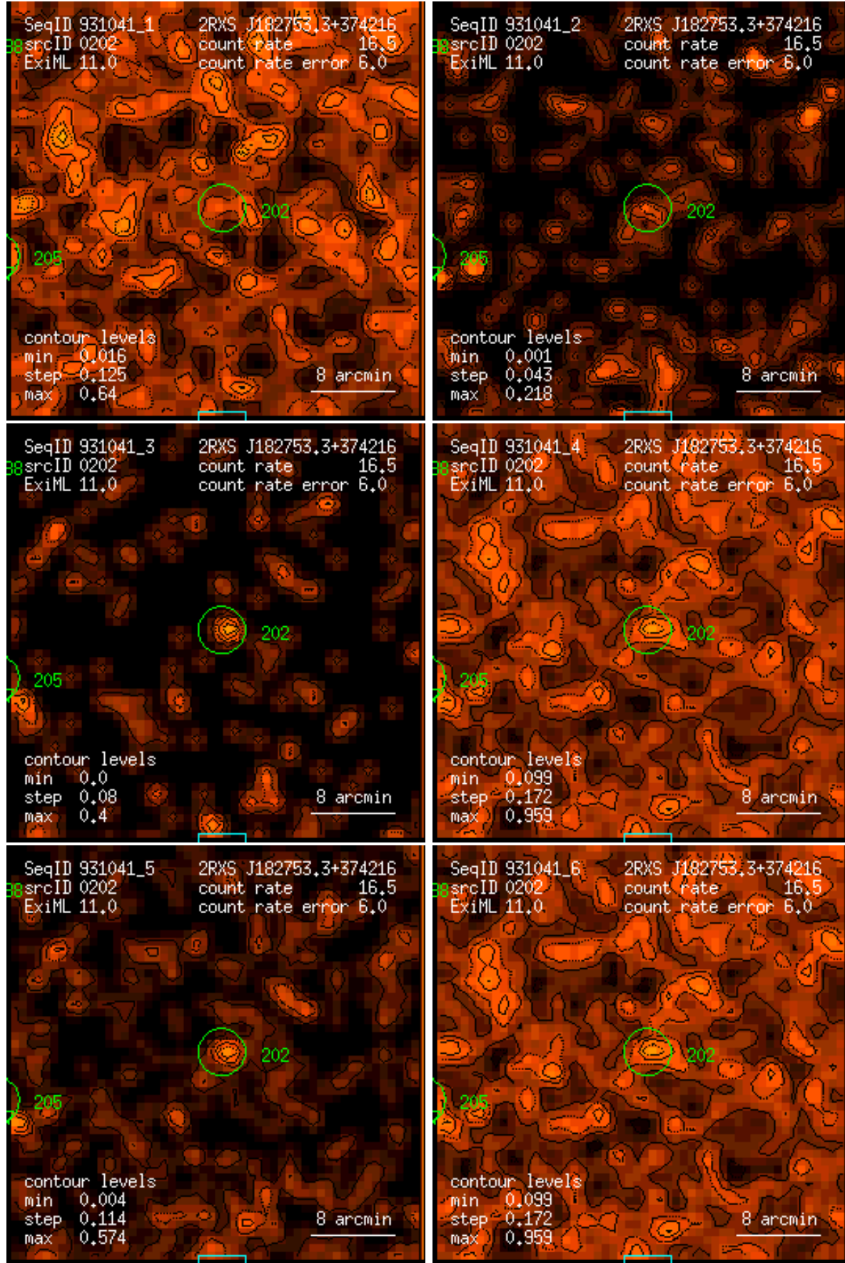
Figure 202: RASS 931041: detection 0202: band rate images, Gaussian filter: (1) PSPC channels 11 – 41, (2) 52 – 90, (3) 91 – 201, (4) 11 – 235, (5) 52 – 201, (6) 11 – 201. Broad band rates in counts/ks. Band rate contour levels in counts/ks/arcmin 2 .
