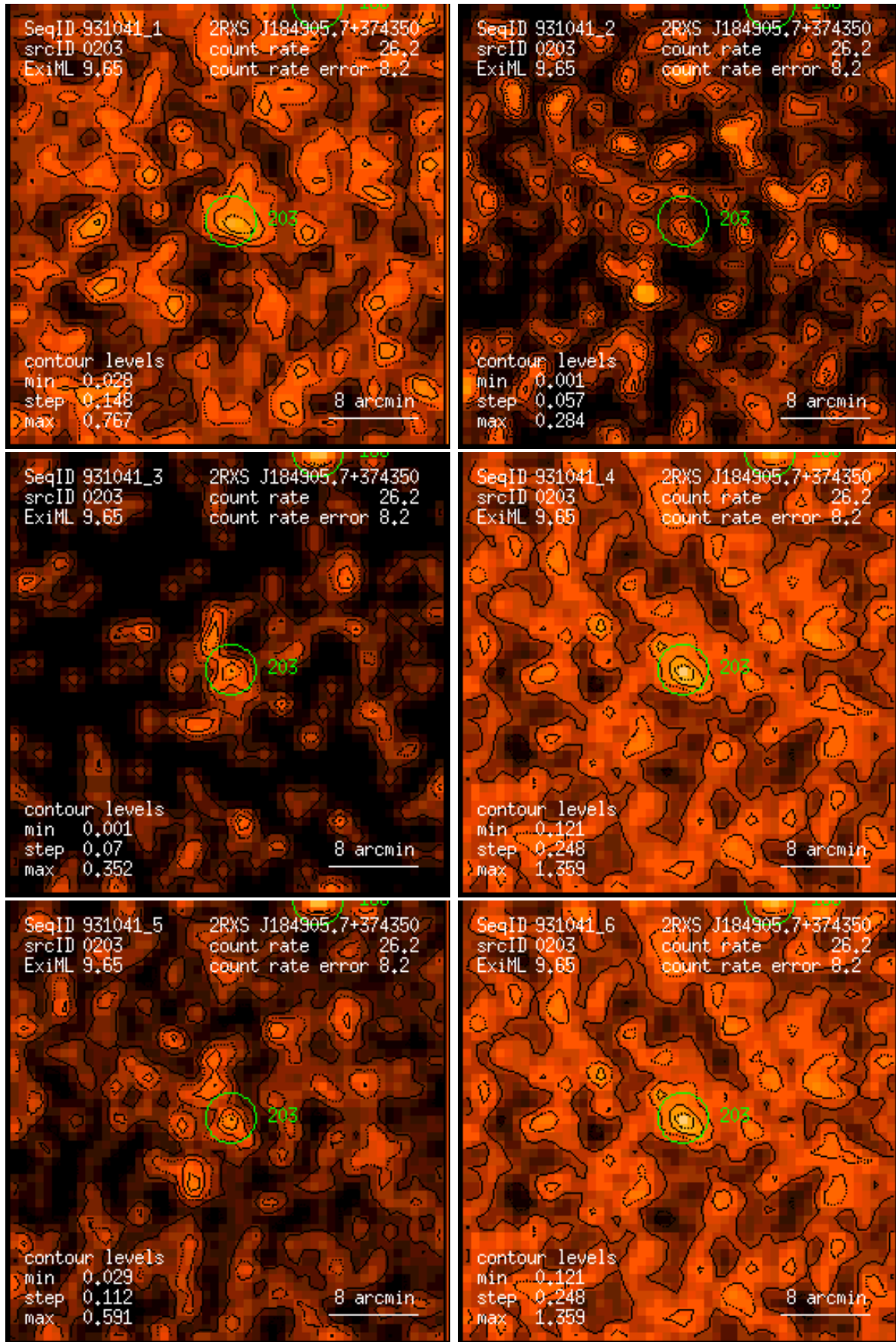
Figure 203: RASS 931041: detection 0203: band rate images, Gaussian filter: (1) PSPC channels 11 – 41, (2) 52 – 90, (3) 91 – 201, (4) 11 – 235, (5) 52 – 201, (6) 11 – 201. Broad band rates in counts/ks. Band rate contour levels in counts/ks/arcmin 2 .
