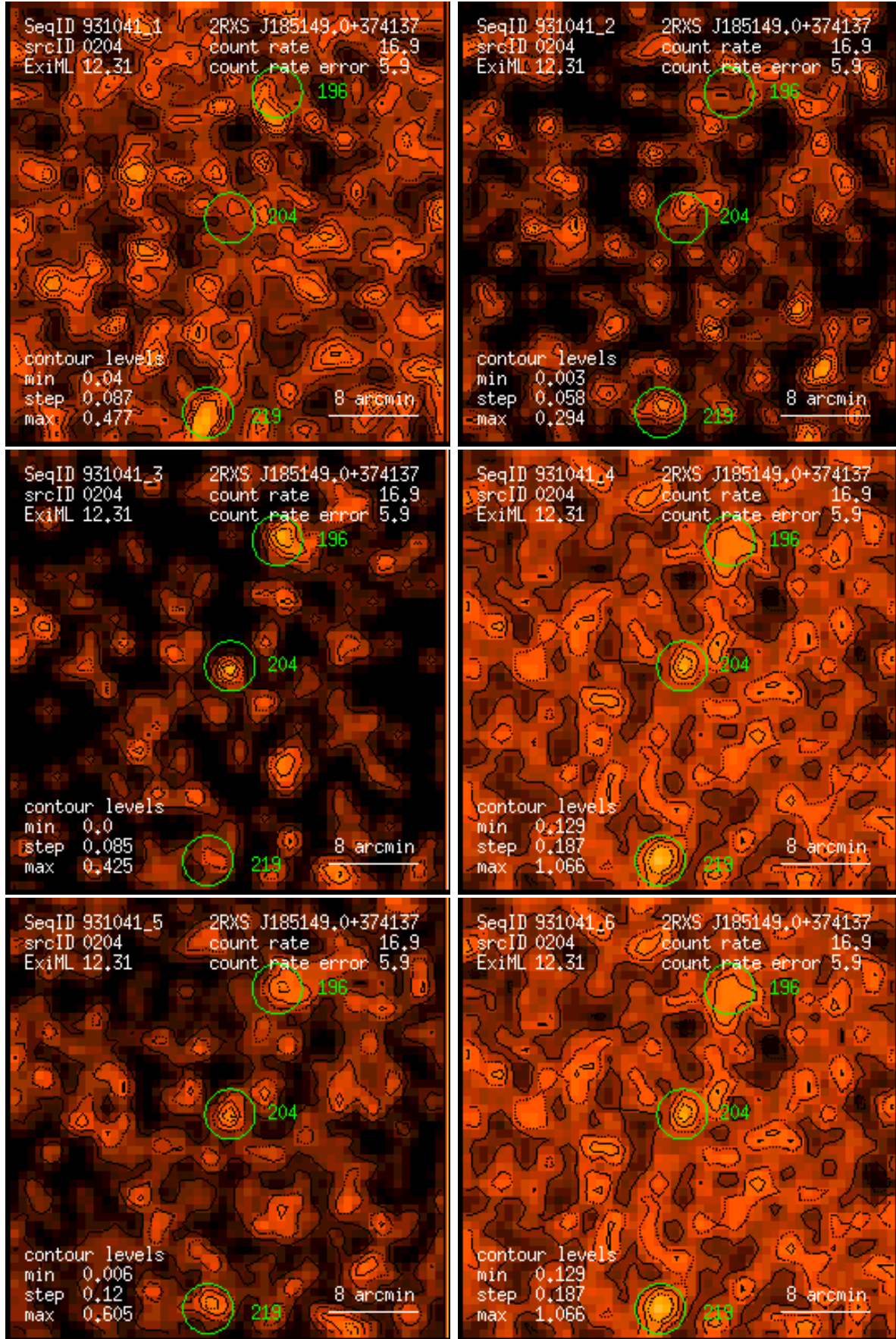
Figure 204: RASS 931041: detection 0204: band rate images, Gaussian filter: (1) PSPC channels 11 – 41, (2) 52 – 90, (3) 91 – 201, (4) 11 – 235, (5) 52 – 201, (6) 11 – 201. Broad band rates in counts/ks. Band rate contour levels in counts/ks/arcmin 2 .
