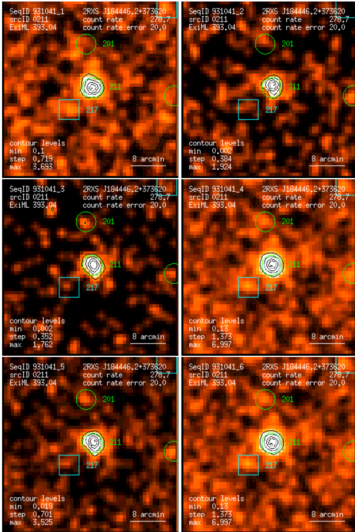
Figure 211: RASS 931041: detection 0211: band rate images, Gaussian filter: (1) PSPC channels 11 – 41, (2) 52 – 90, (3) 91 – 201, (4) 11 – 235, (5) 52 – 201, (6) 11 – 201. Broad band rates in counts/ks. Band rate contour levels in counts/ks/arcmin 2 .
