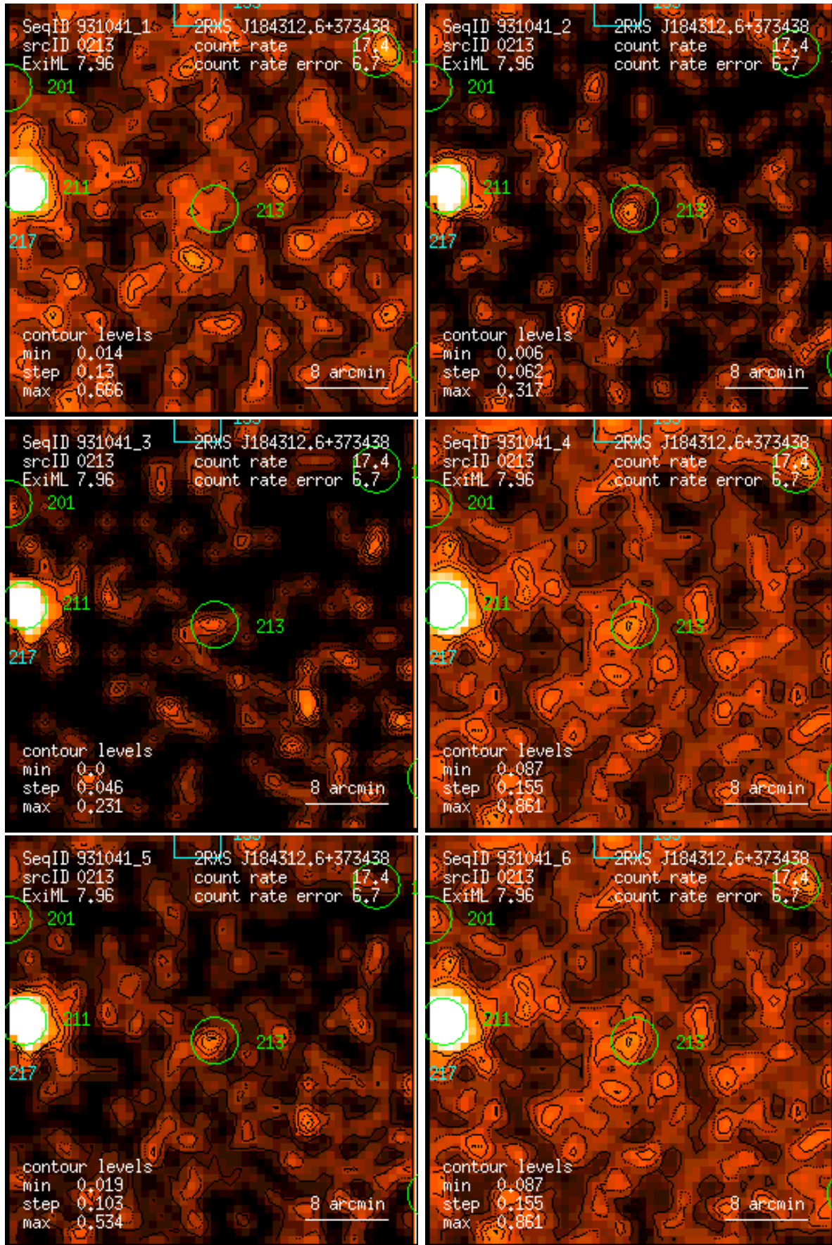
Figure 213: RASS 931041: detection 0213: band rate images, Gaussian filter: (1) PSPC channels 11 – 41, (2) 52 – 90, (3) 91 – 201, (4) 11 – 235, (5) 52 – 201, (6) 11 – 201. Broad band rates in counts/ks. Band rate contour levels in counts/ks/arcmin 2 .
