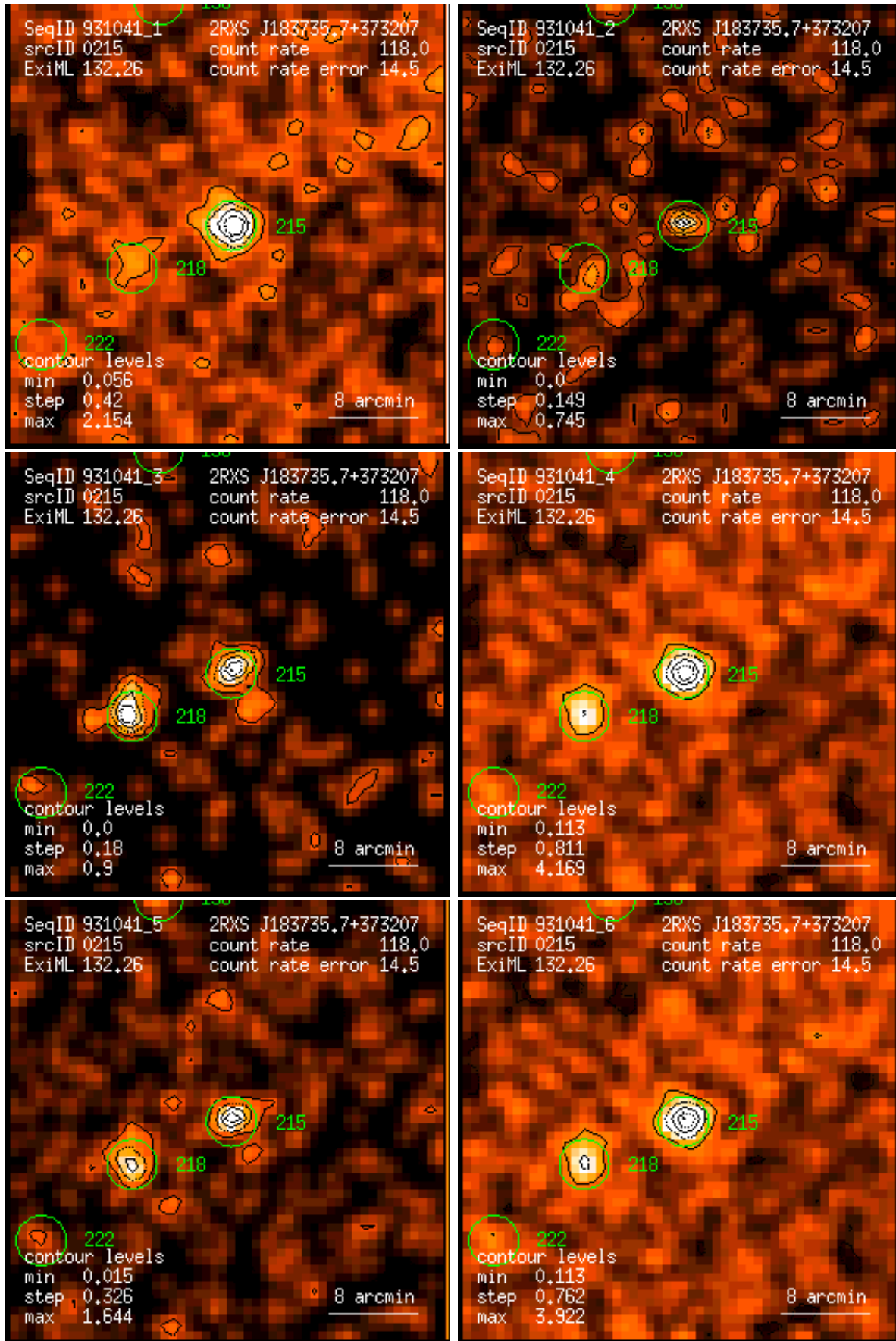
Figure 215: RASS 931041: detection 0215: band rate images, Gaussian filter: (1) PSPC channels 11 – 41, (2) 52 – 90, (3) 91 – 201, (4) 11 – 235, (5) 52 – 201, (6) 11 – 201. Broad band rates in counts/ks. Band rate contour levels in counts/ks/arcmin 2 .
